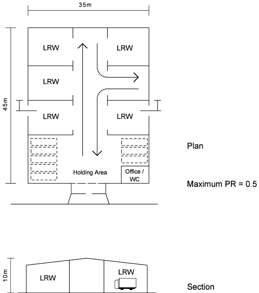
Figure 5.2 Low-Density Purpose-Designed Building
