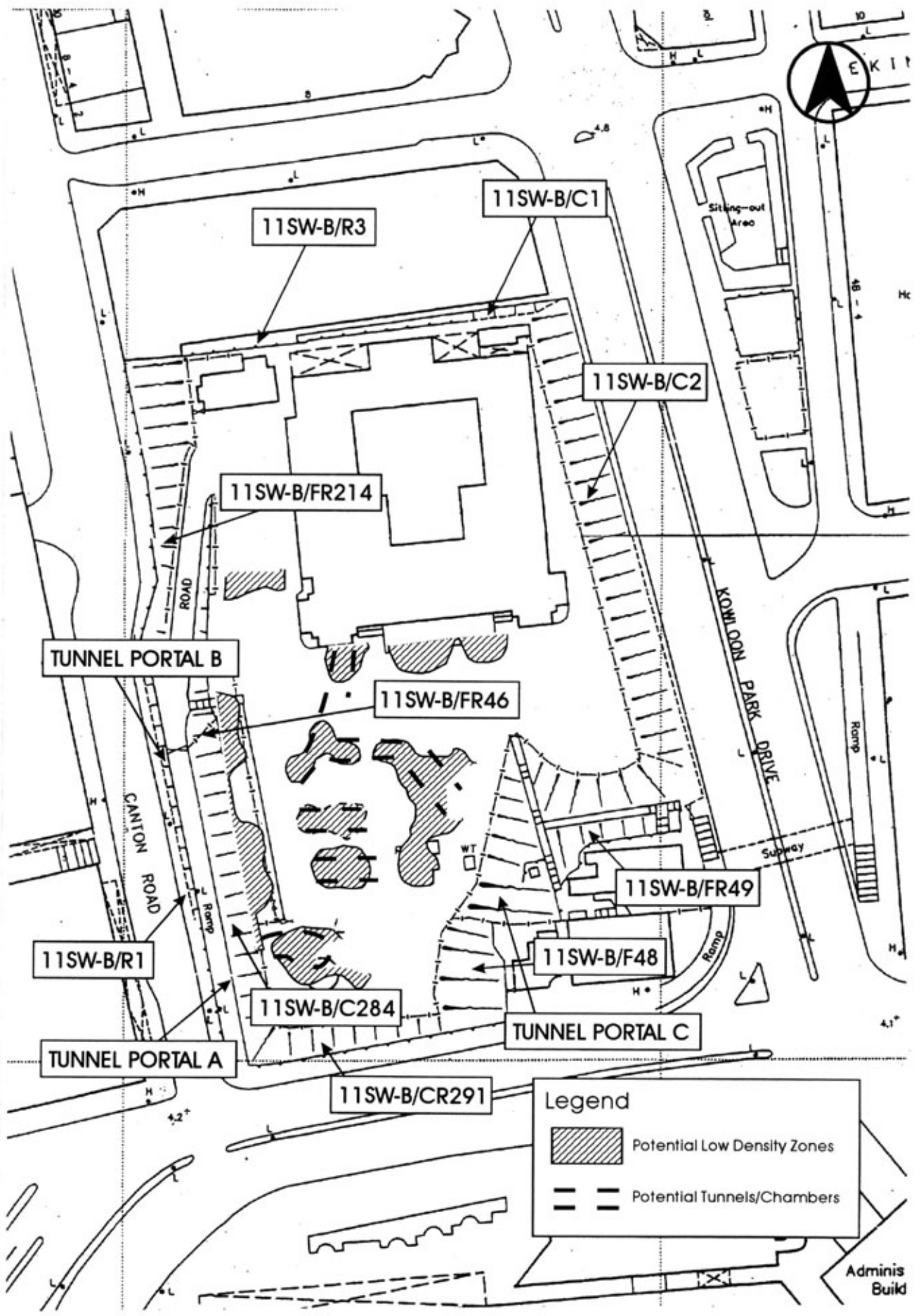
Study on Development Opportunities of the Former Marine Police Headquarters Site in Tsim Sha Tsui Existing Slopes, Tunnel Portals, Potential Density Zones and Potential Tunnels
