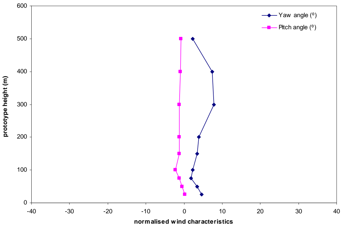
Figure 9b: Mean wind direction, Mong Kok, 45°
