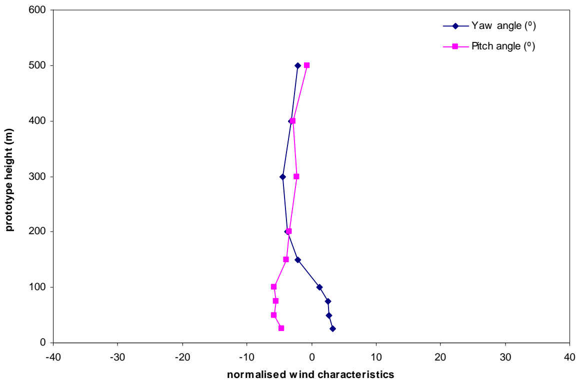
Figure 15b: Mean wind direction, Mong Kok, 180°
