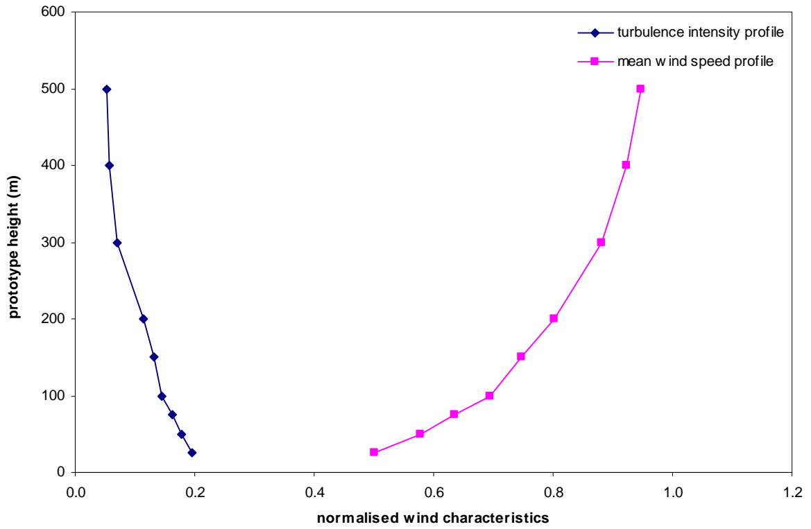
Figure 18a: Wind characteristics, Mong Kok, 247.5°
