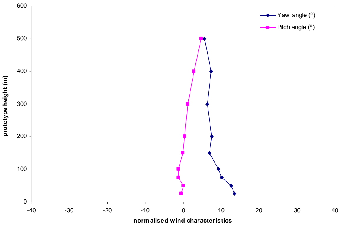
Figure 10b: Mean wind direction, Mong Kok, 67.5°
