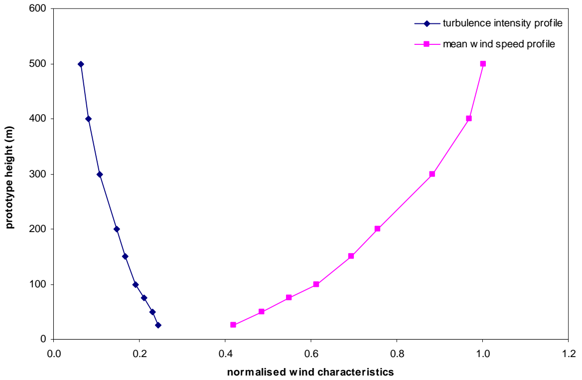
Figure 21a: Wind characteristics, Mong Kok, 315°
