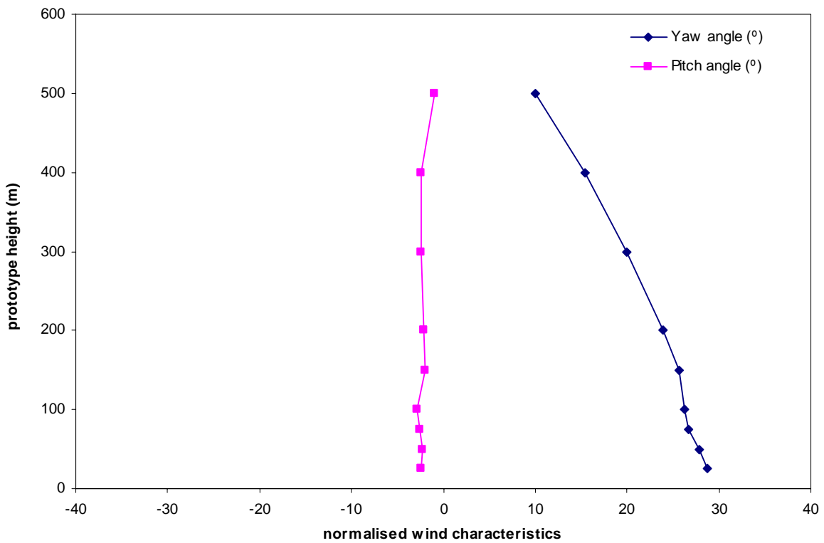
Figure 22b: Mean wind direction, Mong Kok, 337.5°
