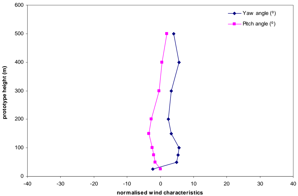
Figure 17b: Mean wind direction, Mong Kok, 225°
