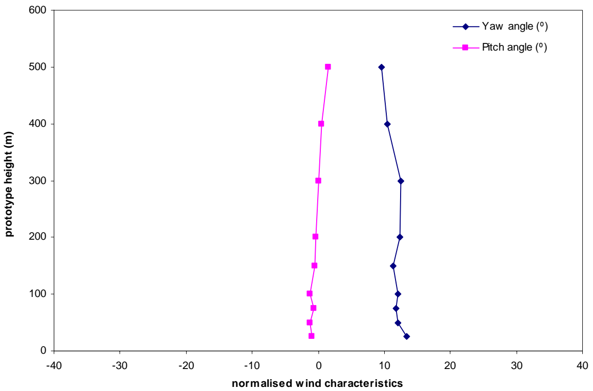
Figure 21b: Mean wind direction, Mong Kok, 315°
