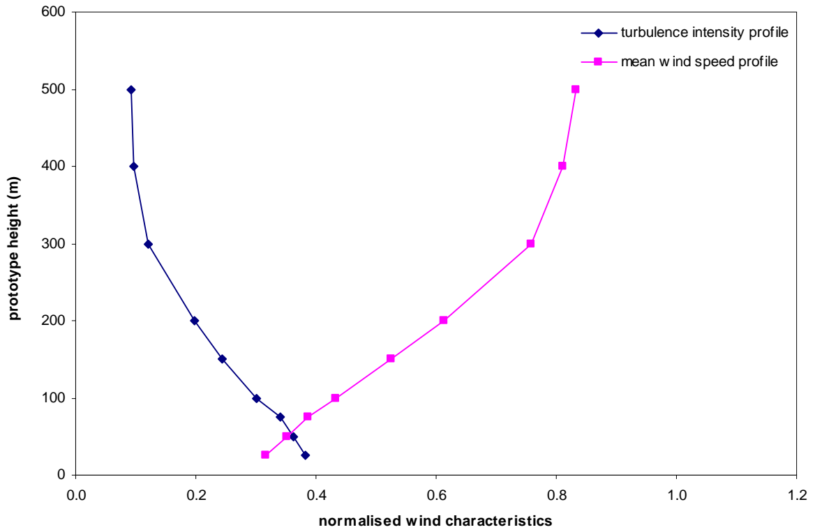
Figure 12a: Wind characteristics, Mong Kok, 112.5°
