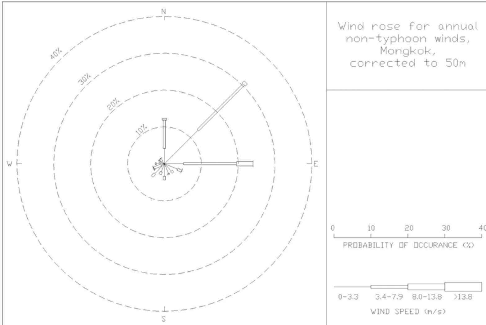
Figure 24: Wind rose for annual, non-typhoon winds for Mong Kok, corrected to 50 m
