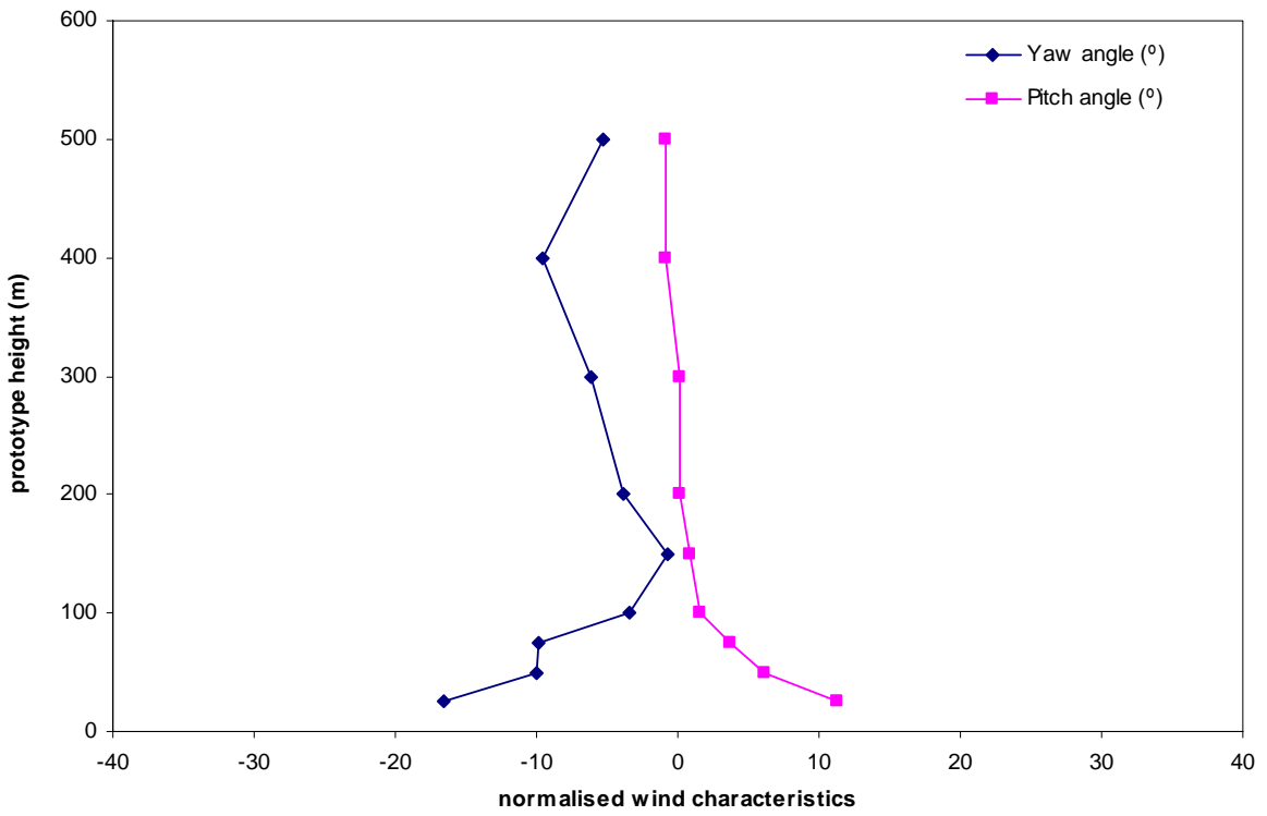
Figure 23b: Mean wind direction, Mong Kok, 360°
