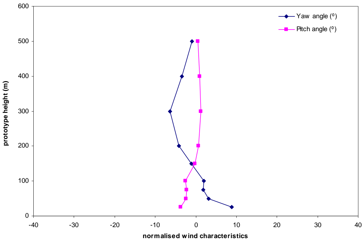
Figure 13b: Mean wind direction, Mong Kok, 135°
