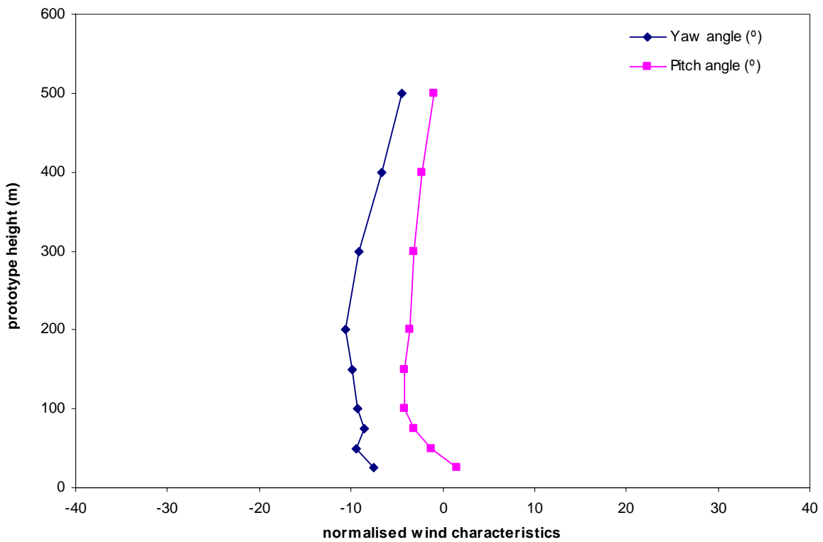
Figure 16b: Mean wind direction, Mong Kok, 202.5°
