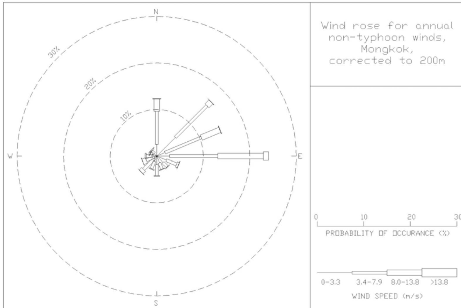
Figure 26: Wind rose for annual, non-typhoon winds for Mong Kok, corrected to 200 m
