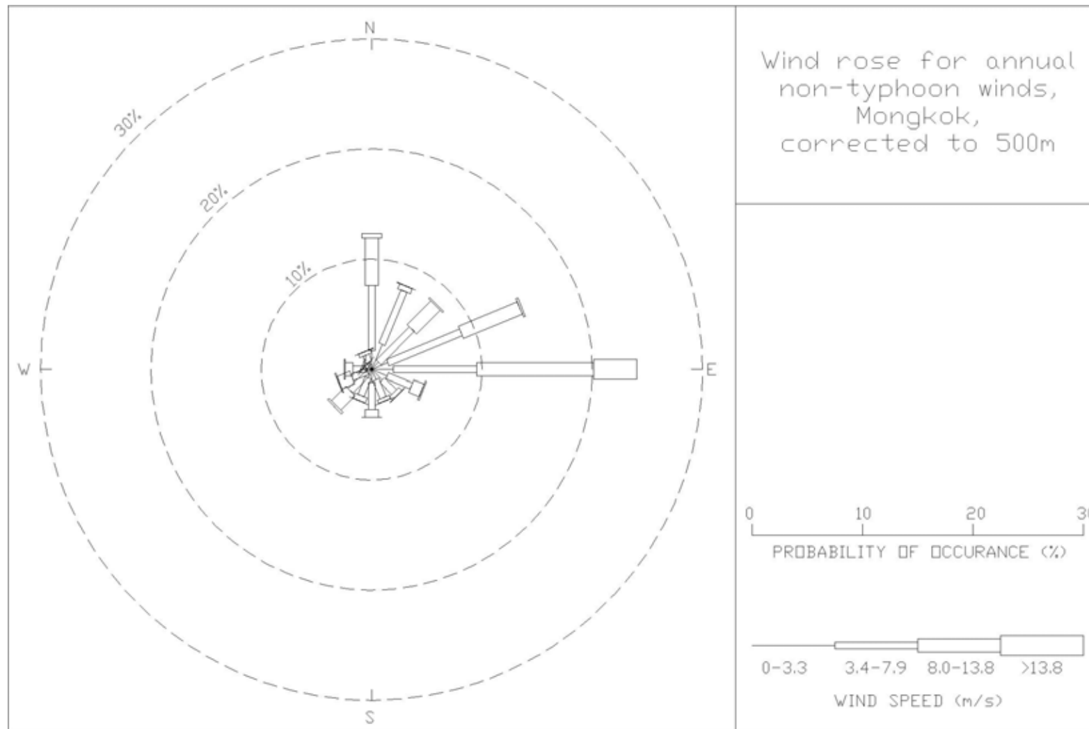
Figure 27: Wind rose for annual, non-typhoon winds for Mong Kok, corrected to 500 m
