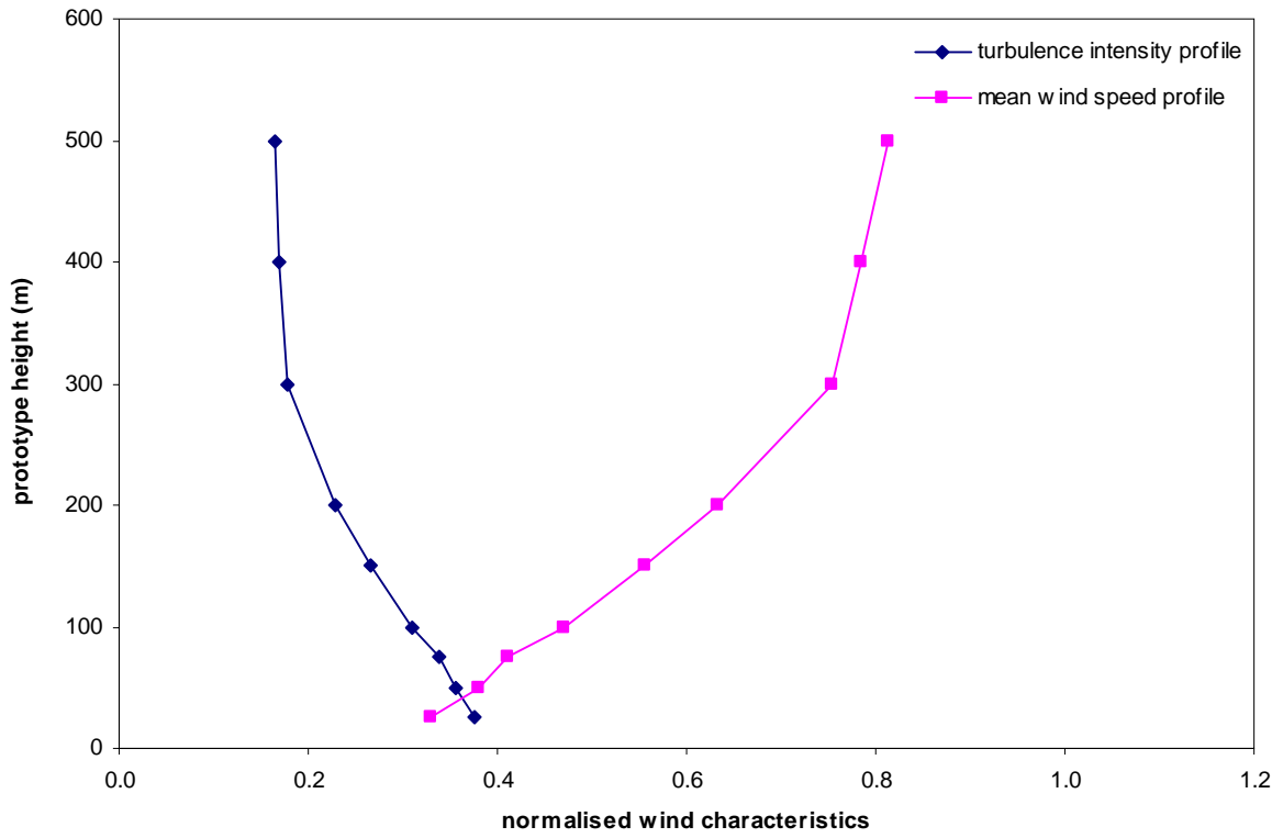
Figure 16a: Wind characteristics, Mong Kok, 202.5°
