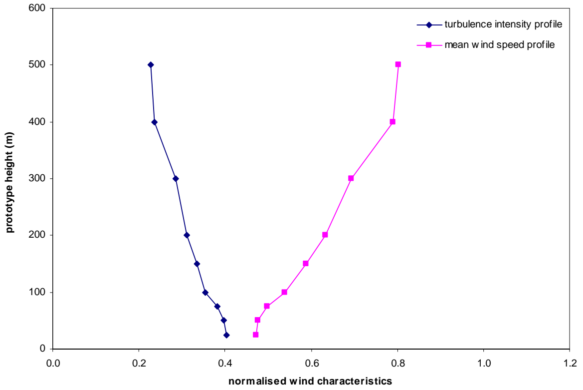
Figure 23a: Wind characteristics, Mong Kok, 360°
