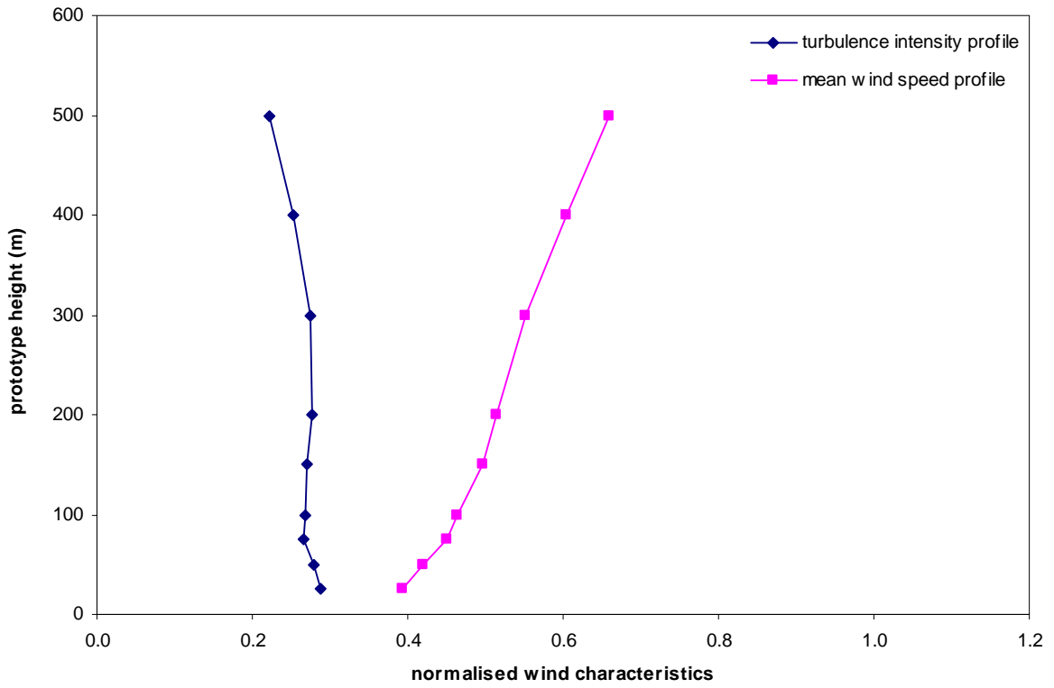
Figure 8a: Wind characteristics, Mong Kok, 22.5°
