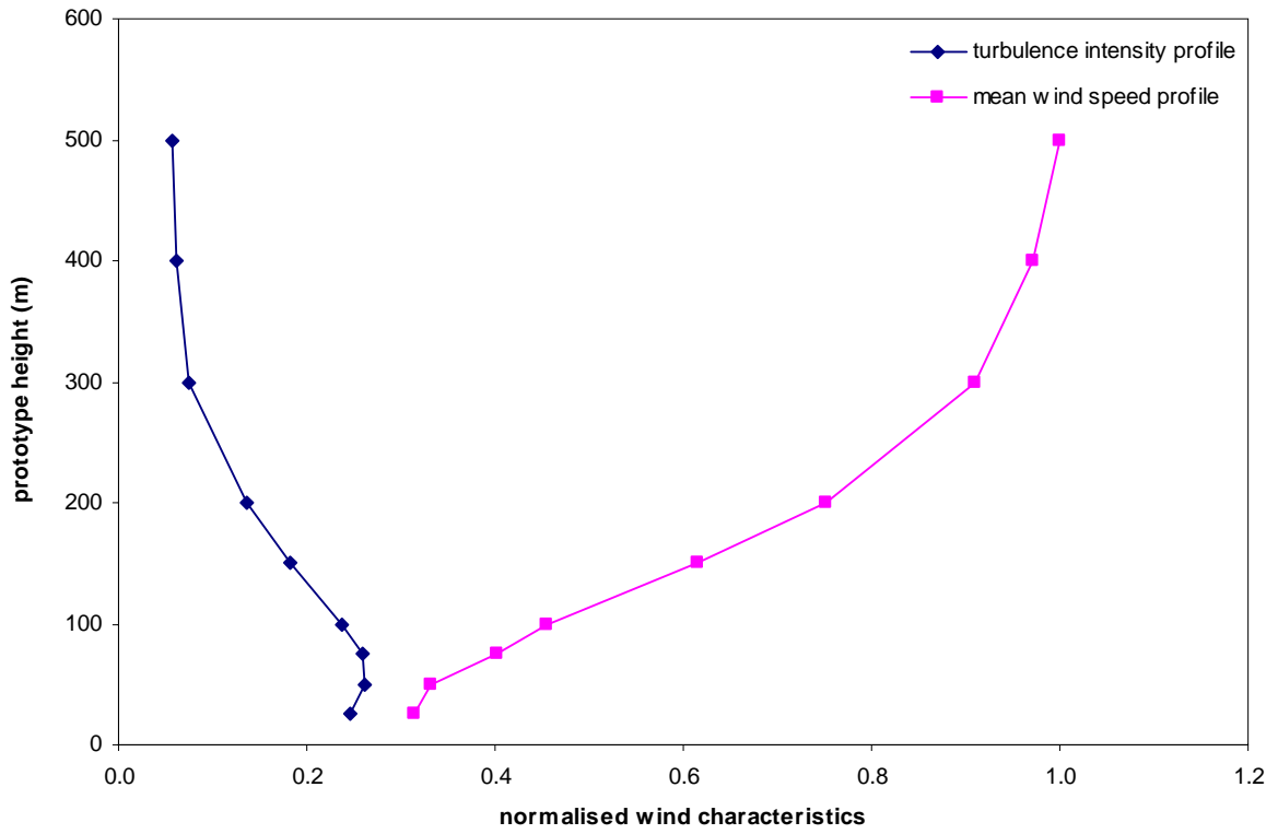
Figure 19a: Wind characteristics, Mong Kok, 270°
