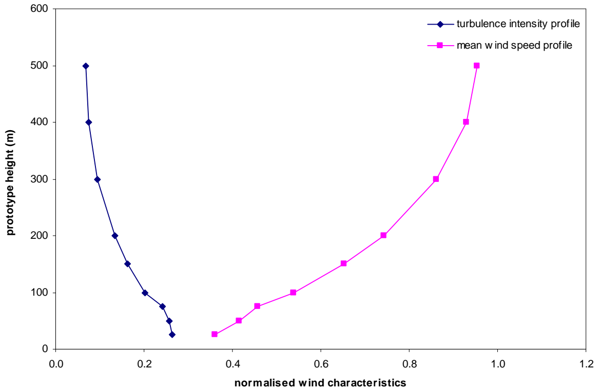
Figure 20a: Wind characteristics, Mong Kok, 292.5°
