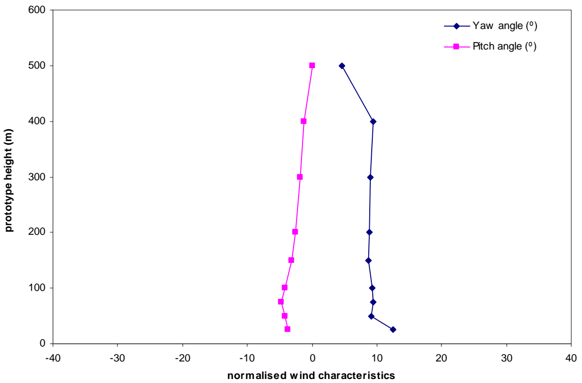
Figure 14b: Mean wind direction, Mong Kok, 157.5°
