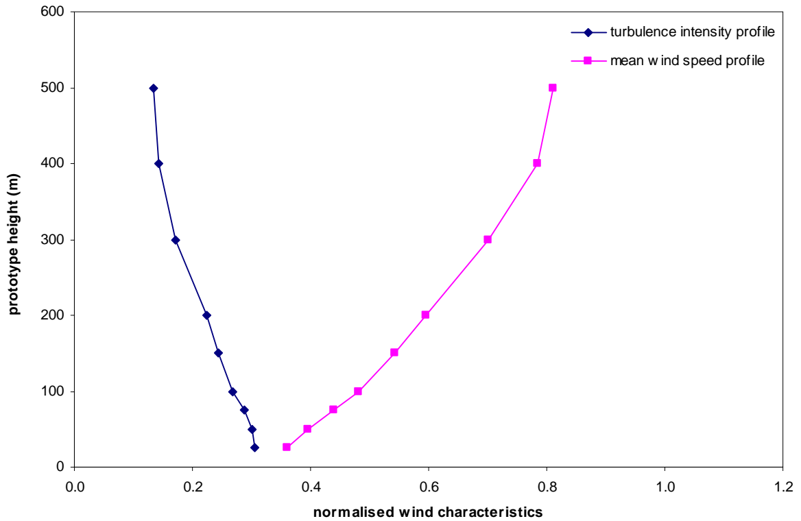
Figure 13a: Wind characteristics, Mong Kok, 135°
