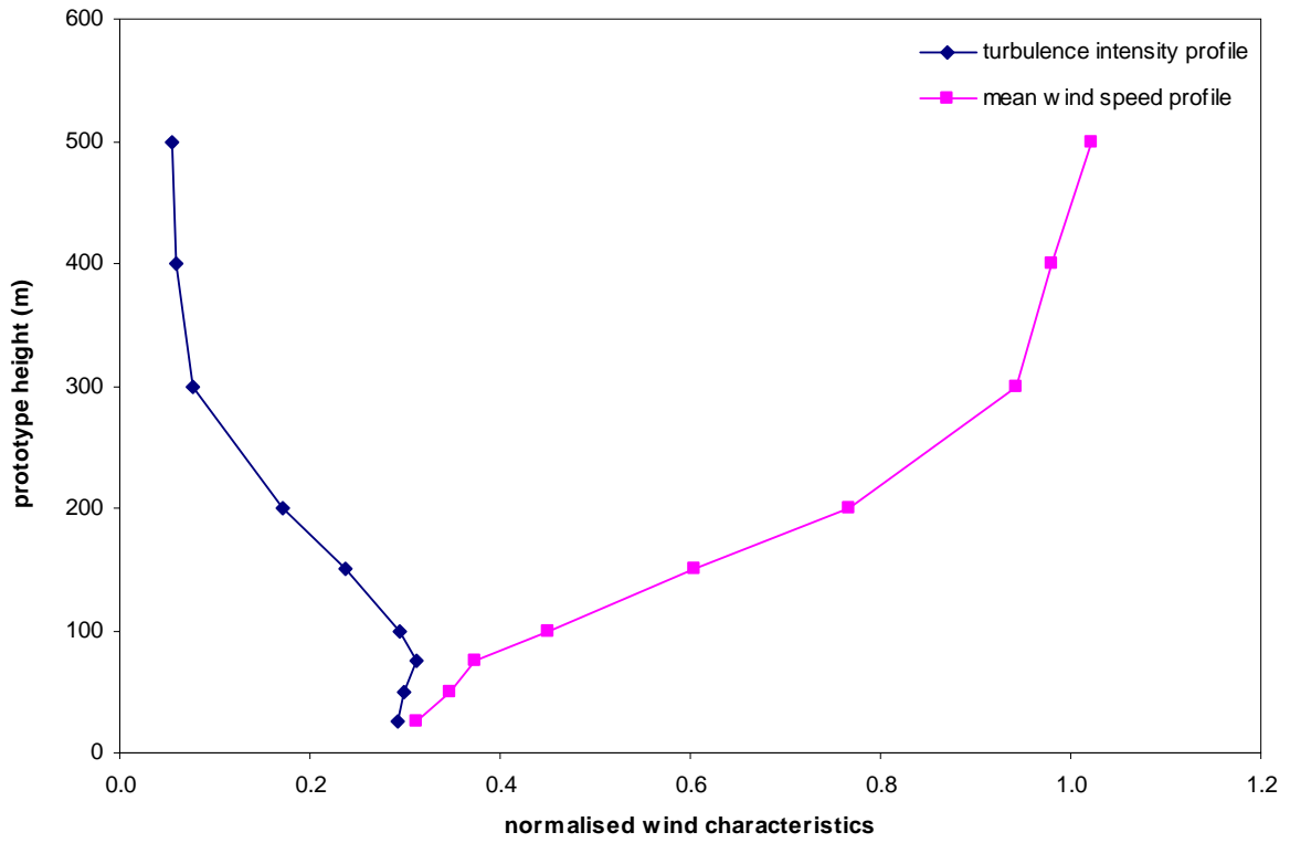
Figure 17a: Wind characteristics, Mong Kok, 225°
