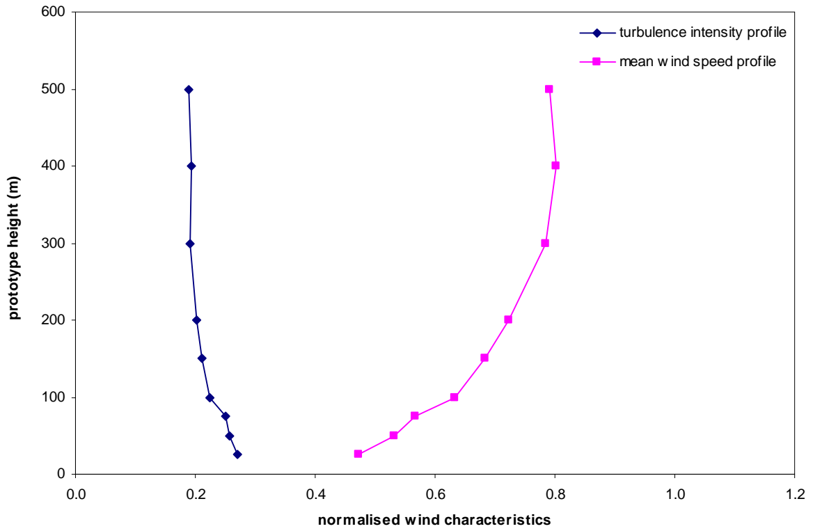
Figure 22a: Wind characteristics, Mong Kok, 337.5°
