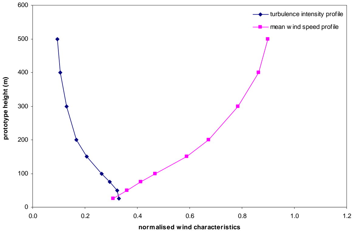
Figure 14a: Wind characteristics, Mong Kok, 157.5°
