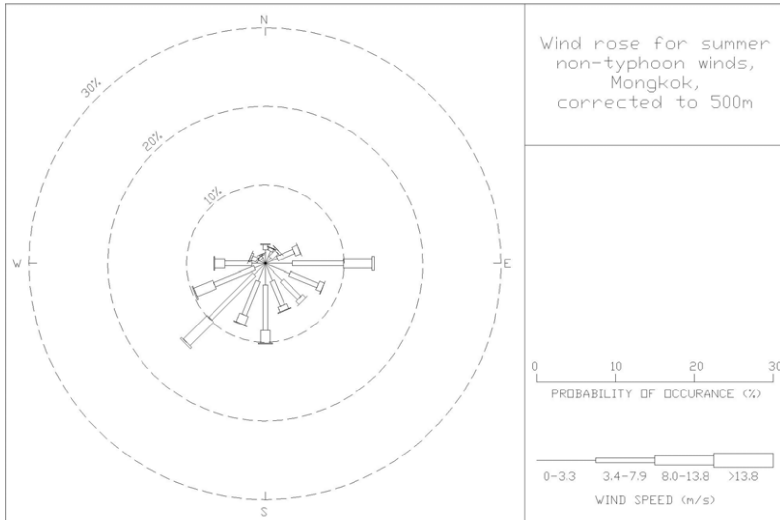
Figure 31: Wind rose for summer, non-typhoon winds for Mong Kok, corrected to 500 m
