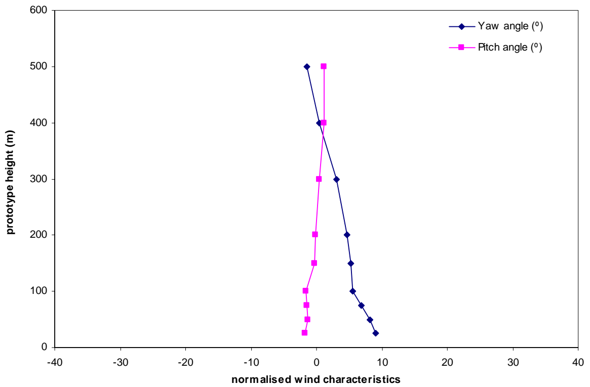
Figure 11b: Mean wind direction, Mong Kok, 90°
