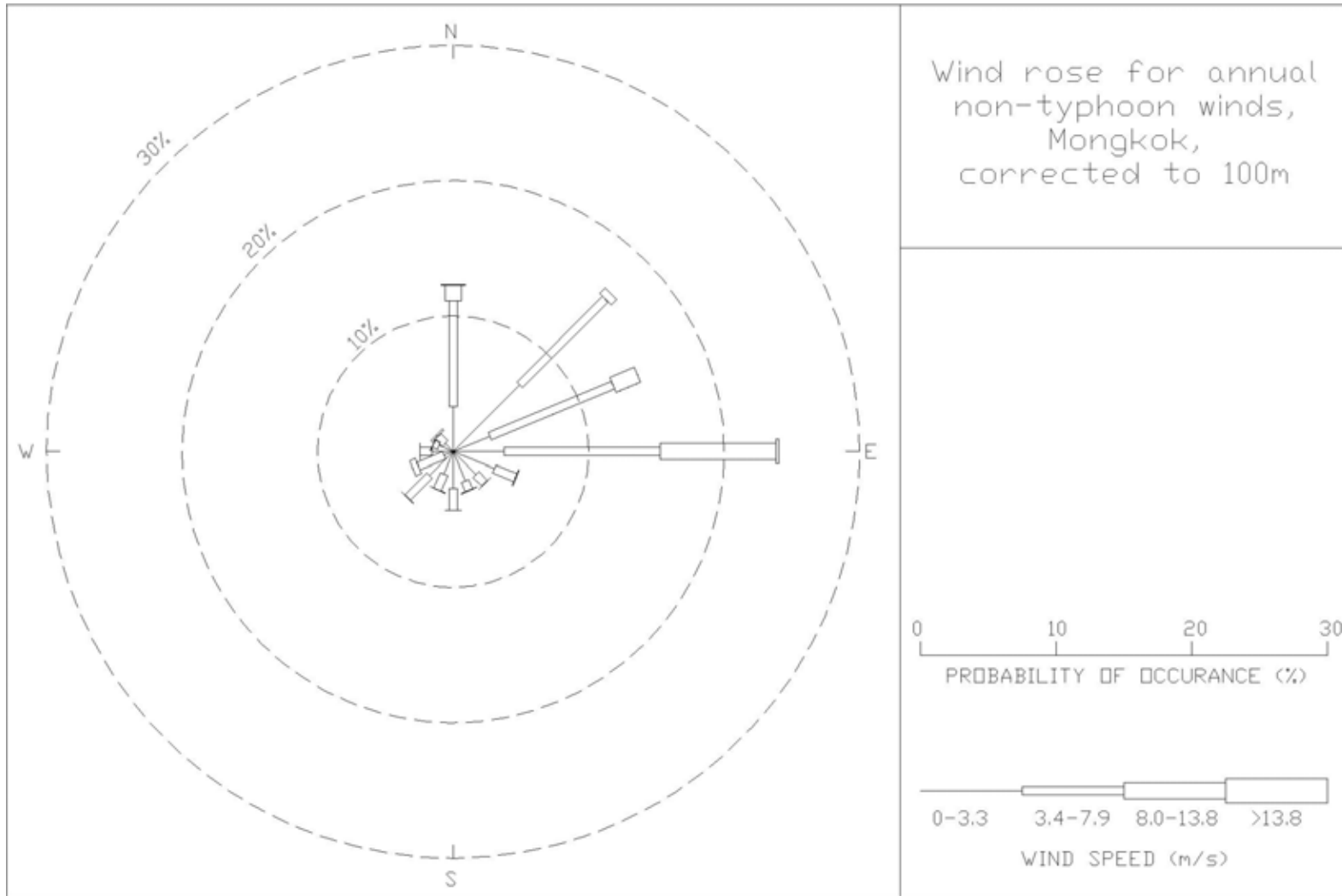
Figure 25: Wind rose for annual, non-typhoon winds for Mong Kok, corrected to 100 m
