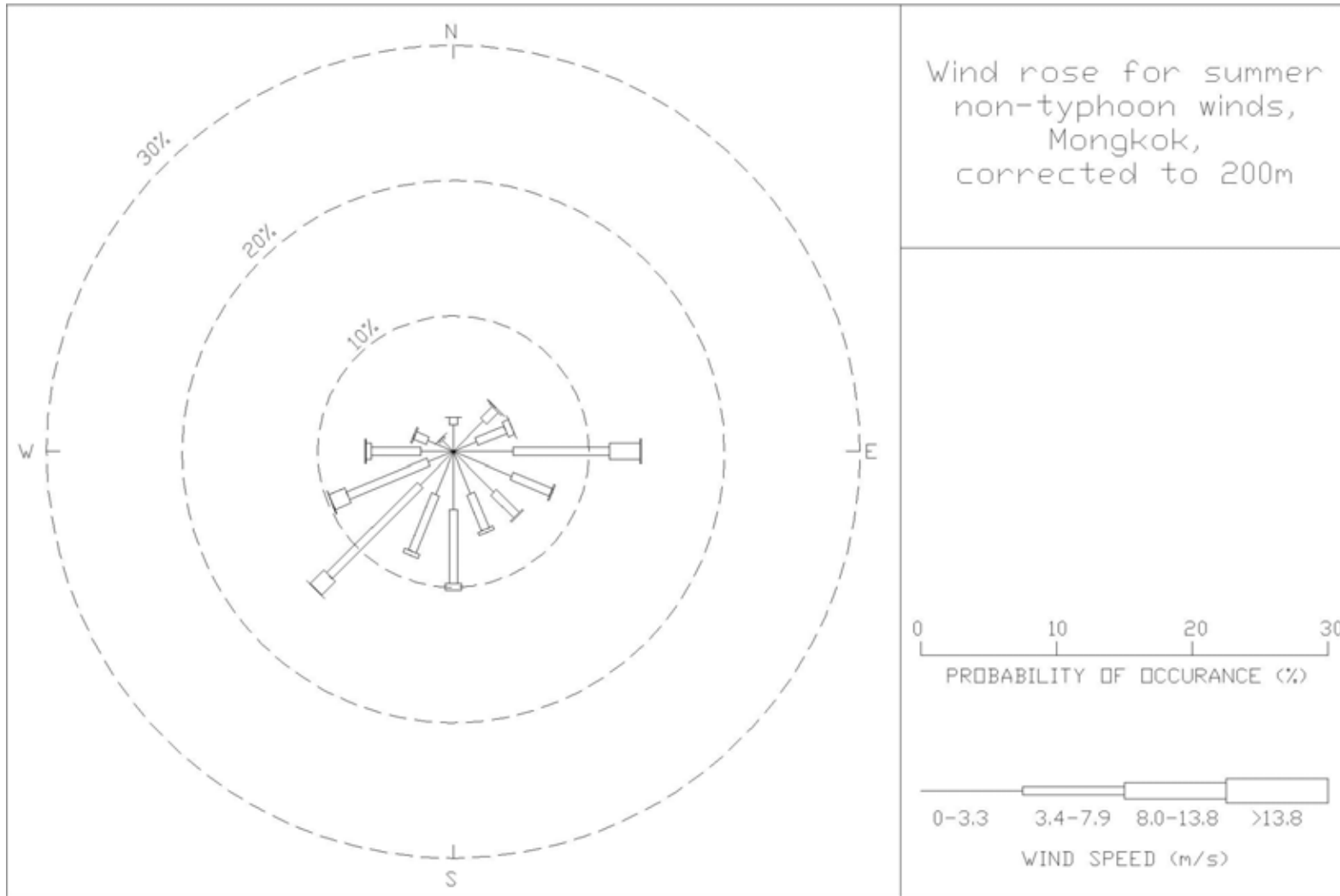
Figure 30: Wind rose for summer, non-typhoon winds for Mong Kok, corrected to 200 m
