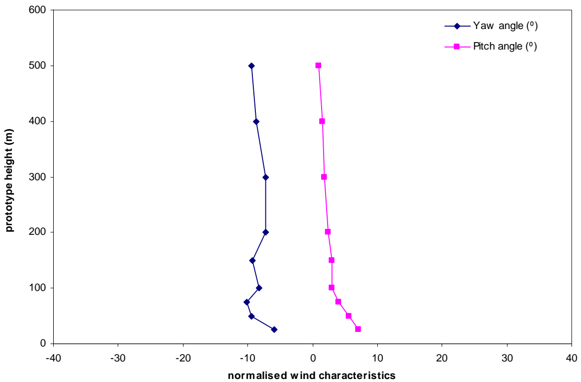
Figure 12b: Mean wind direction, Mong Kok, 112.5°
