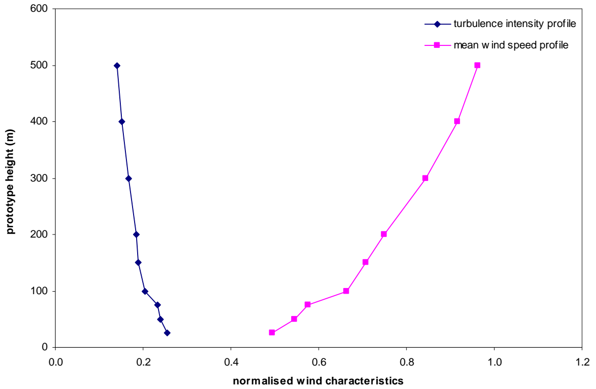
Figure 9a: Wind characteristics, Mong Kok, 45°
