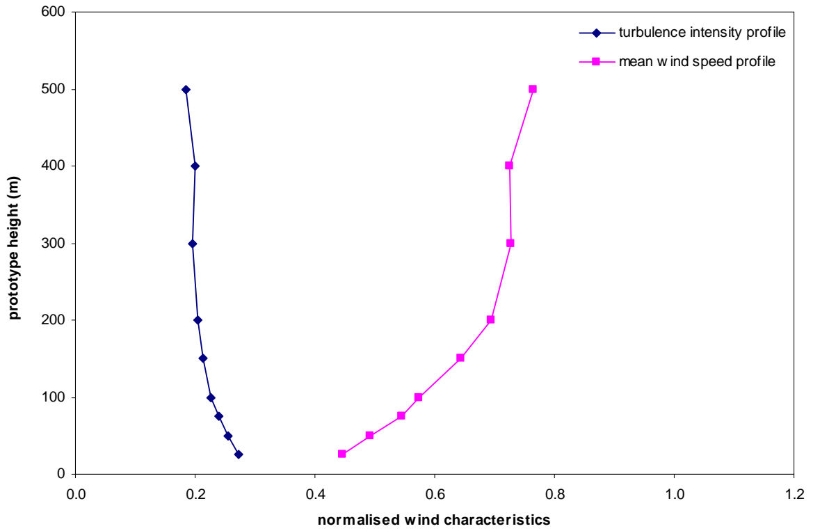
Figure 10a: Wind characteristics, Mong Kok, 67.5°
