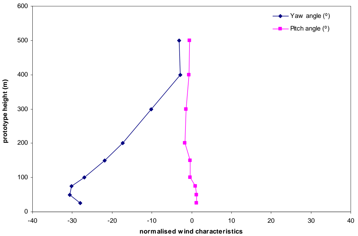
Figure 8b: Mean wind direction, Mong Kok, 22.5°
