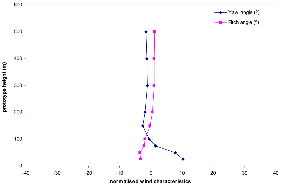
Figure 19b: Mean wind direction, Mong Kok, 270°
