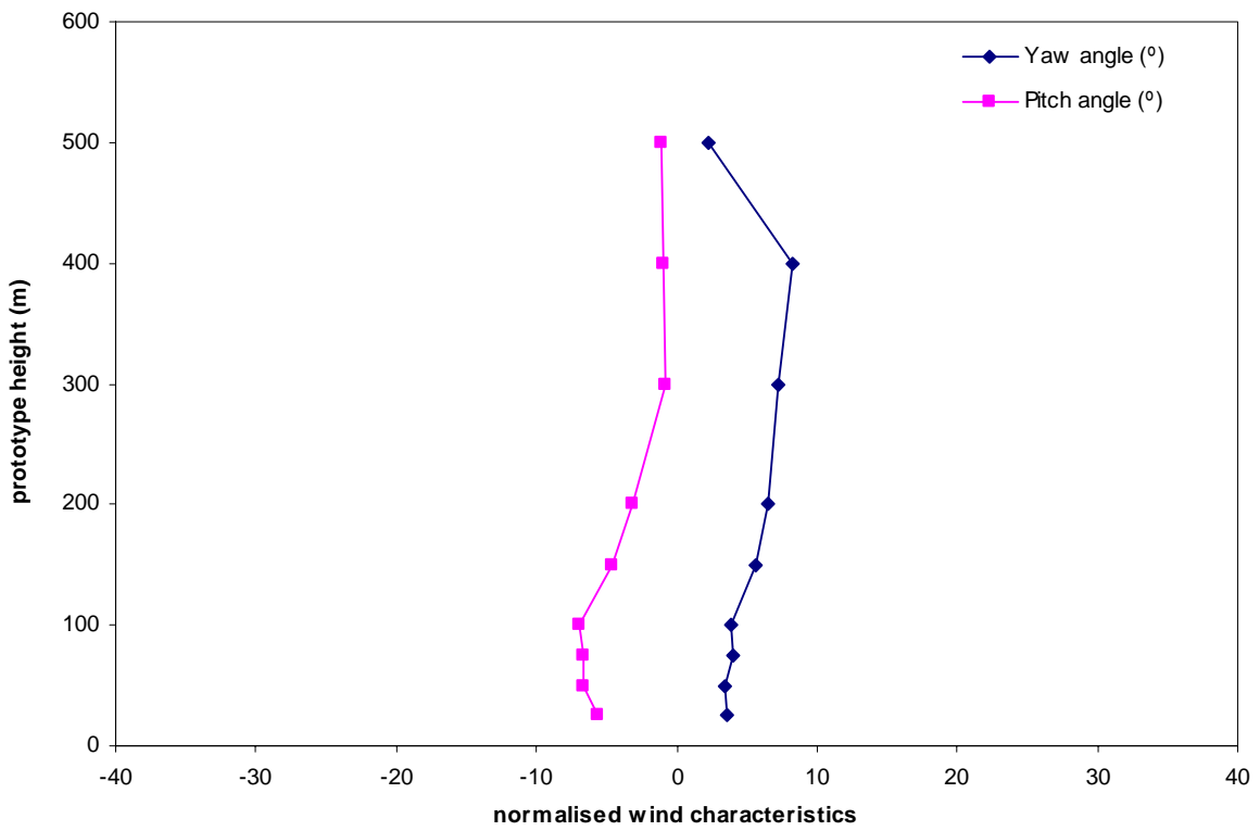
Figure 18b: Mean wind direction, Mong Kok, 247.5°
