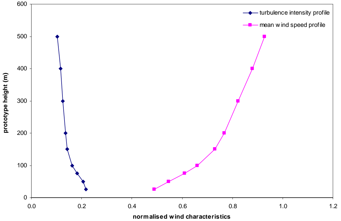
Figure 11a: Wind characteristics, Mong Kok, 90°
