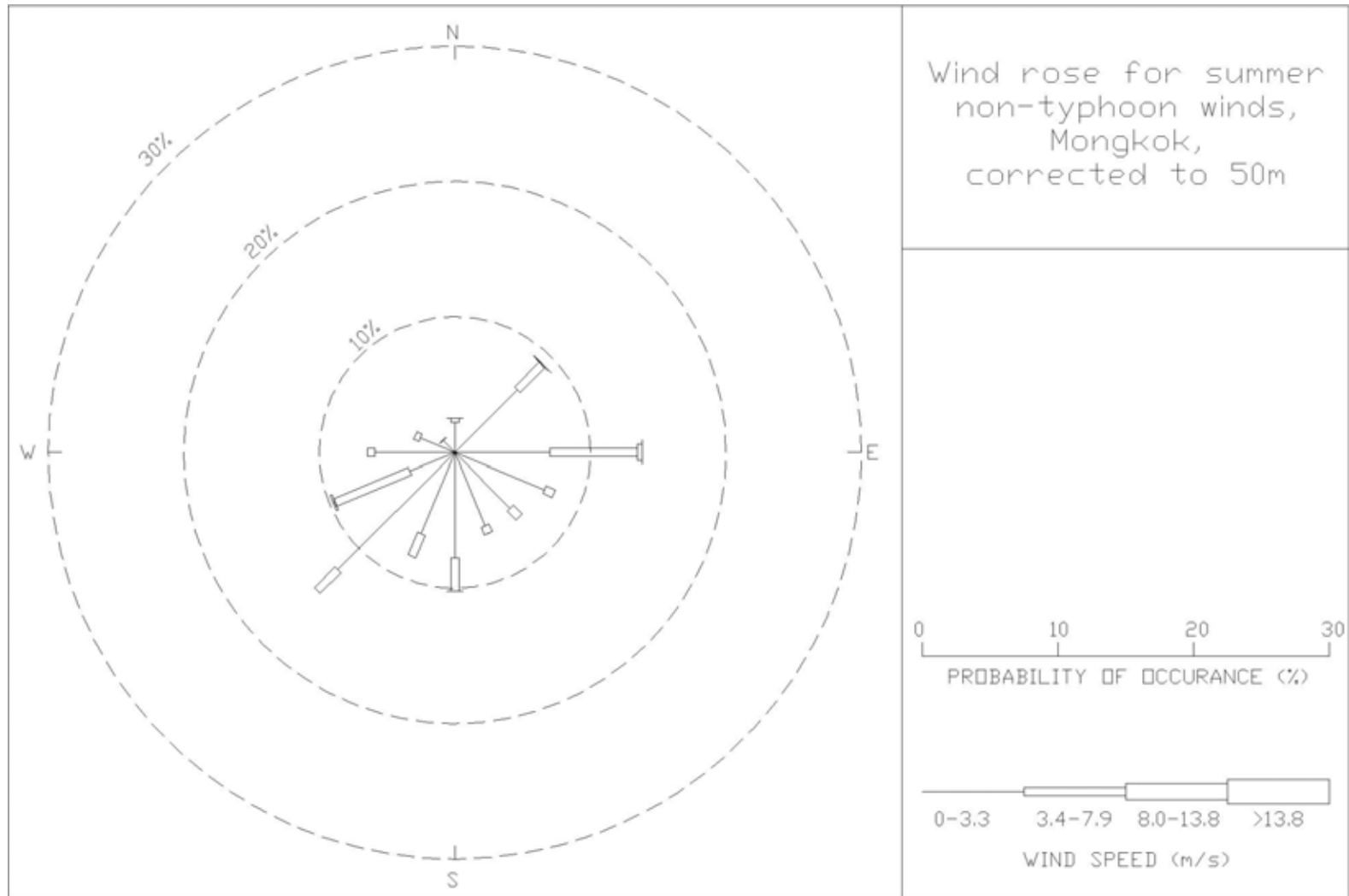
Figure 28: Wind rose for summer, non-typhoon winds for Mong Kok, corrected to 50 m
