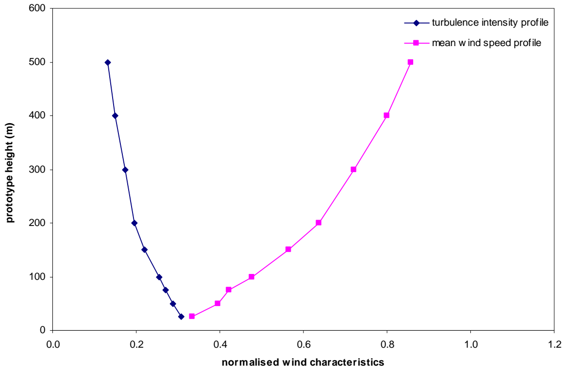
Figure 15a: Wind characteristics, Mong Kok, 180°
