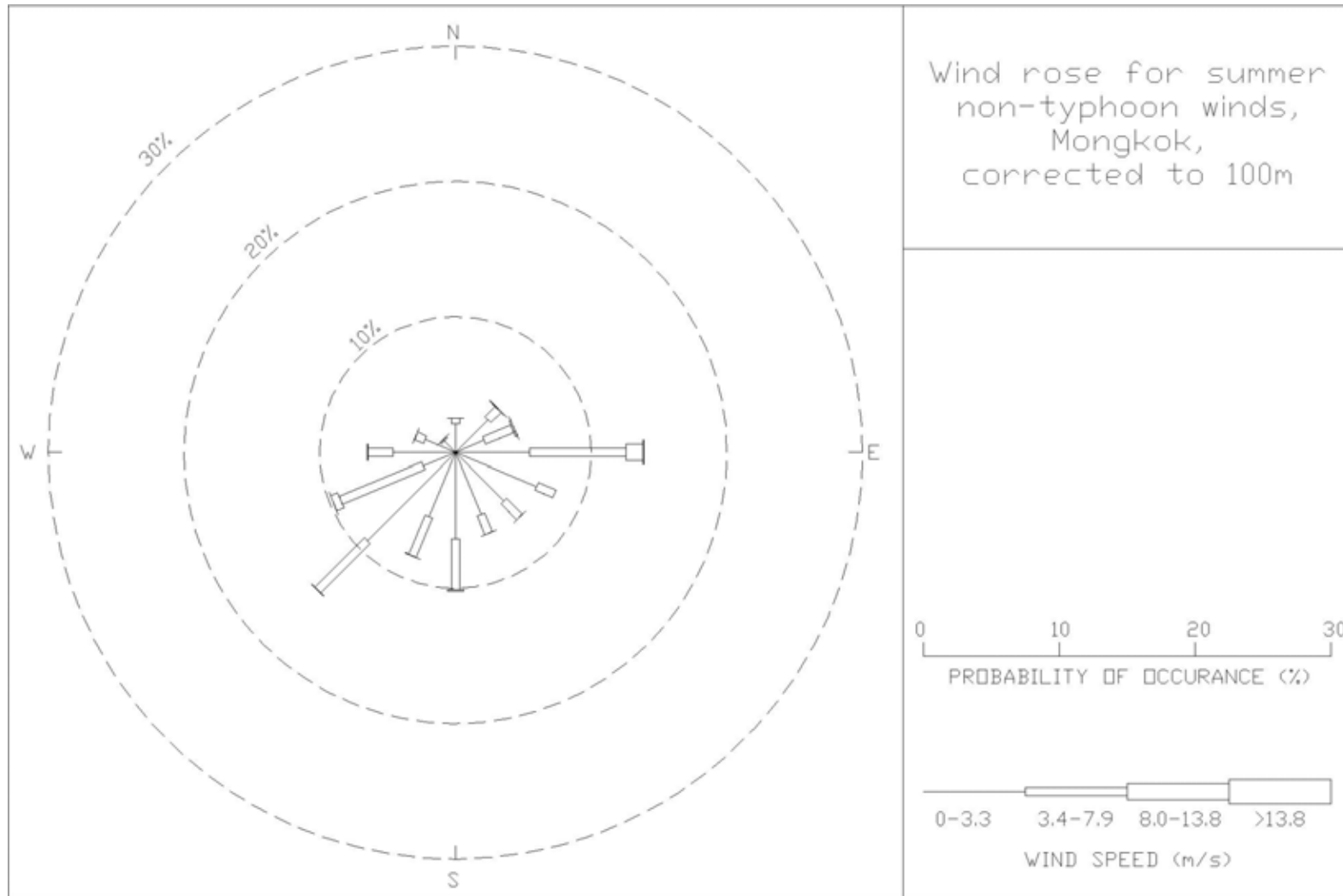
Figure 29: Wind rose for summer, non-typhoon winds for Mong Kok, corrected to 100 m
