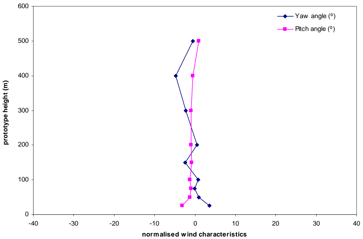
Figure 20b: Mean wind direction, Mong Kok, 292.5°
