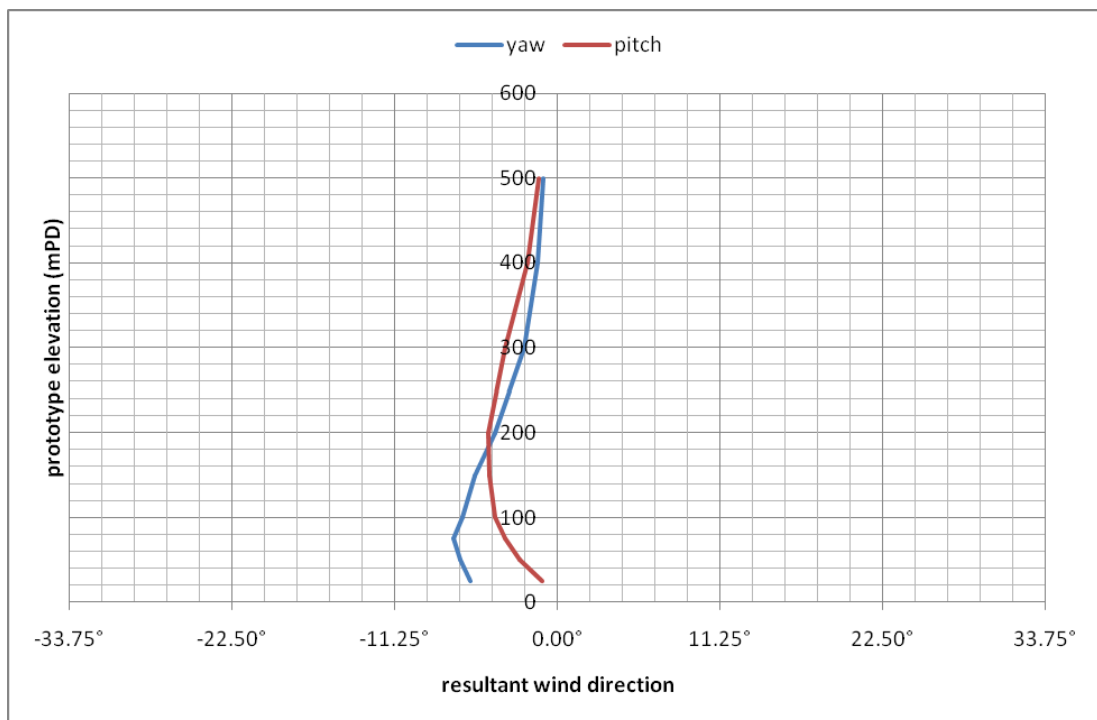
Figure 9b: Mean wind directions for Tseung Kwan O, 22.5°
