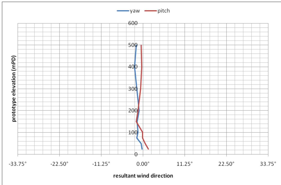
Figure 17b: Mean wind directions for Tseung Kwan O, 202.5°
