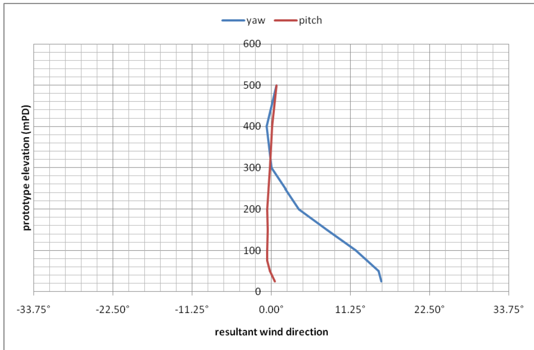
Figure 15b: Mean wind directions for Tseung Kwan O, 157.5°
