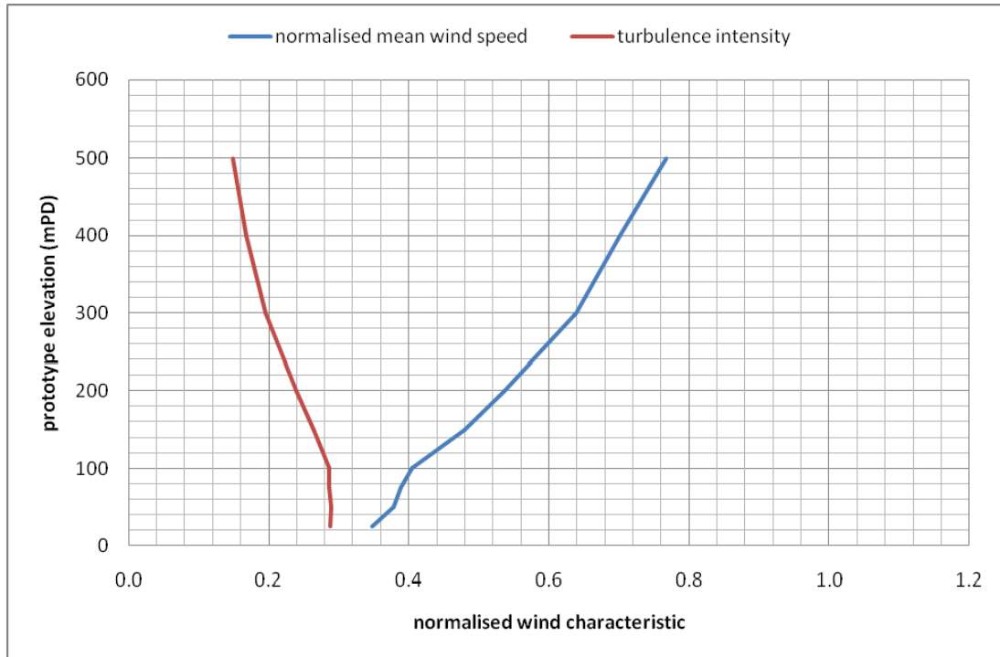
Figure 17a: Wind characteristics for Tseung Kwan O, 202.5°
