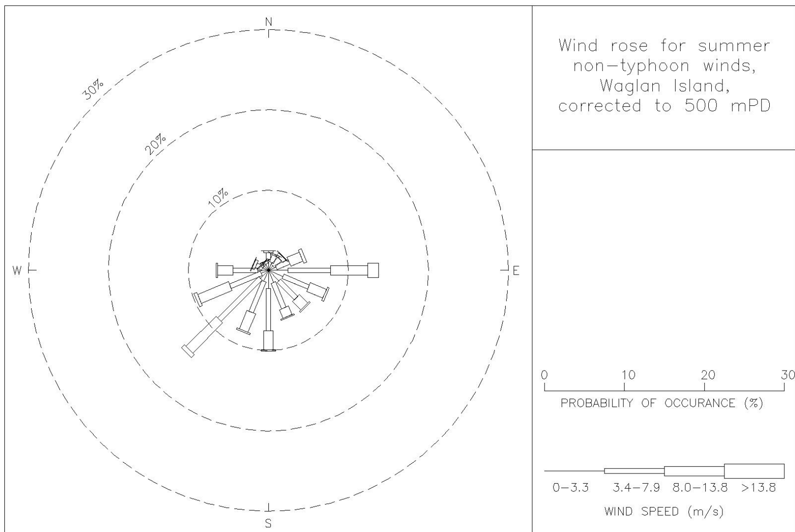
Figure 4: Wind rose for summer non-typhoon winds, Waglan Island corrected to 500 mPD above open sea, 1953-2006
