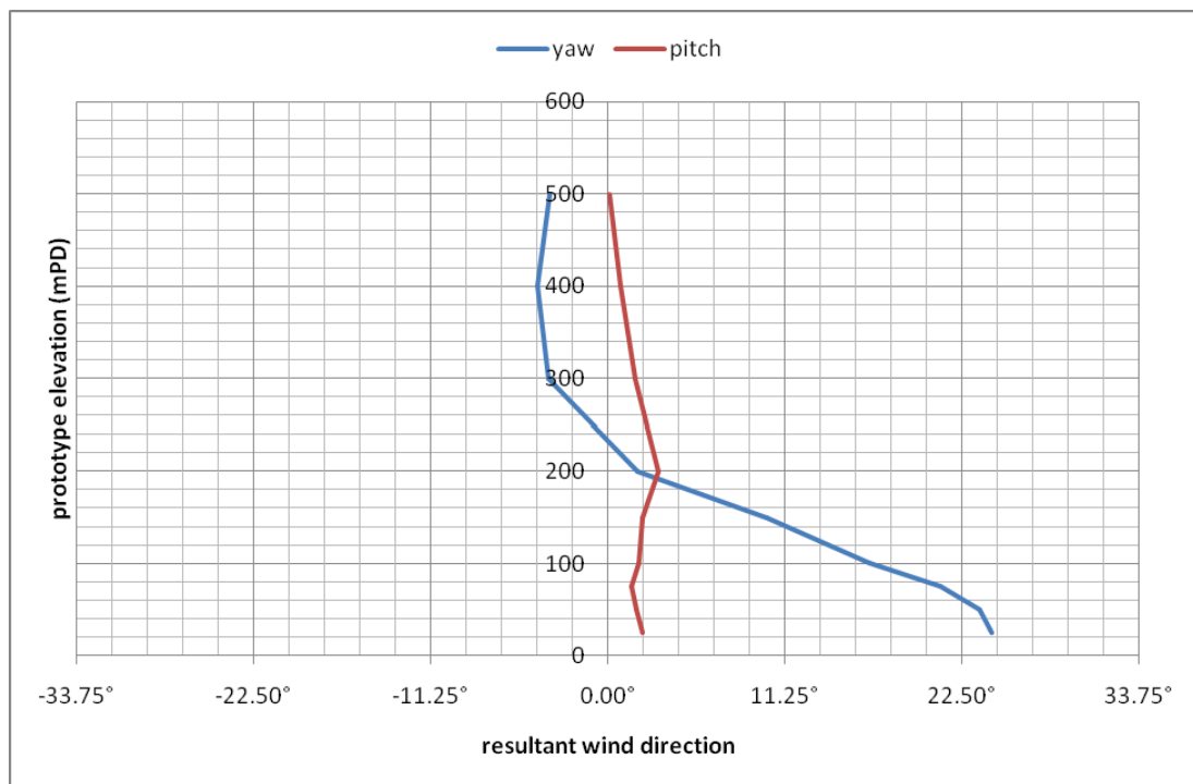
Figure 24b: Mean wind directions for Tseung Kwan O, 360°
