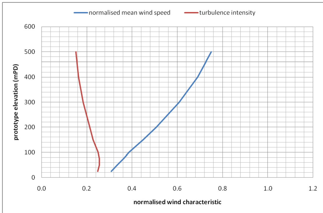
Figure 18a: Wind characteristics for Tseung Kwan O, 225°
