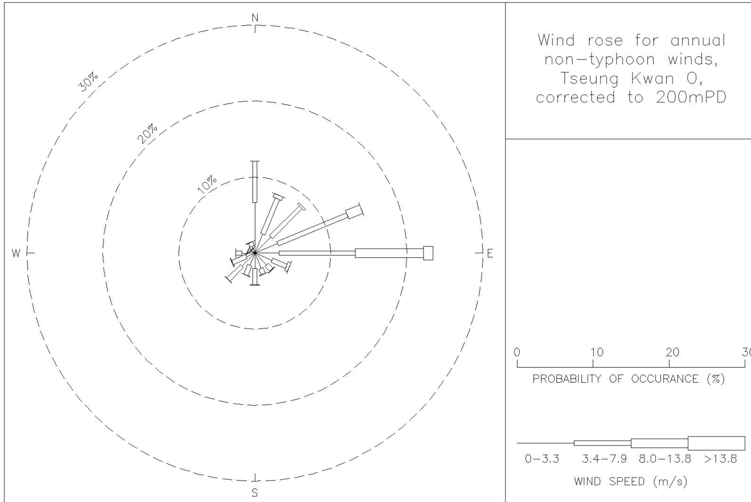
Figure 27: Wind rose for annual, non-typhoon winds for Tseung Kwan O, corrected to 200 mPD
