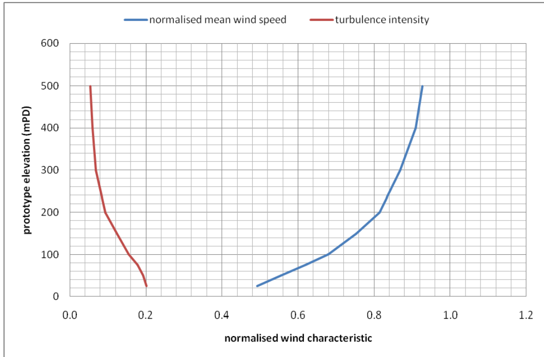
Figure 12a: Wind characteristics for Tseung Kwan O, 90°
