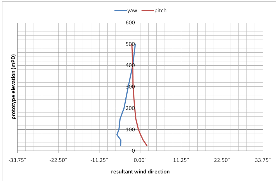
Figure 21b: Mean wind directions for Tseung Kwan O, 292.5°
