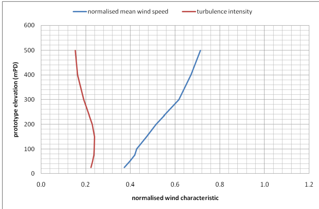
Figure 23a: Wind characteristics for Tseung Kwan O, 337.5°
