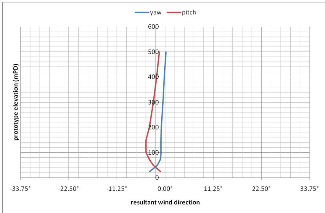
Figure 16b: Mean wind directions for Tseung Kwan O, 180°
