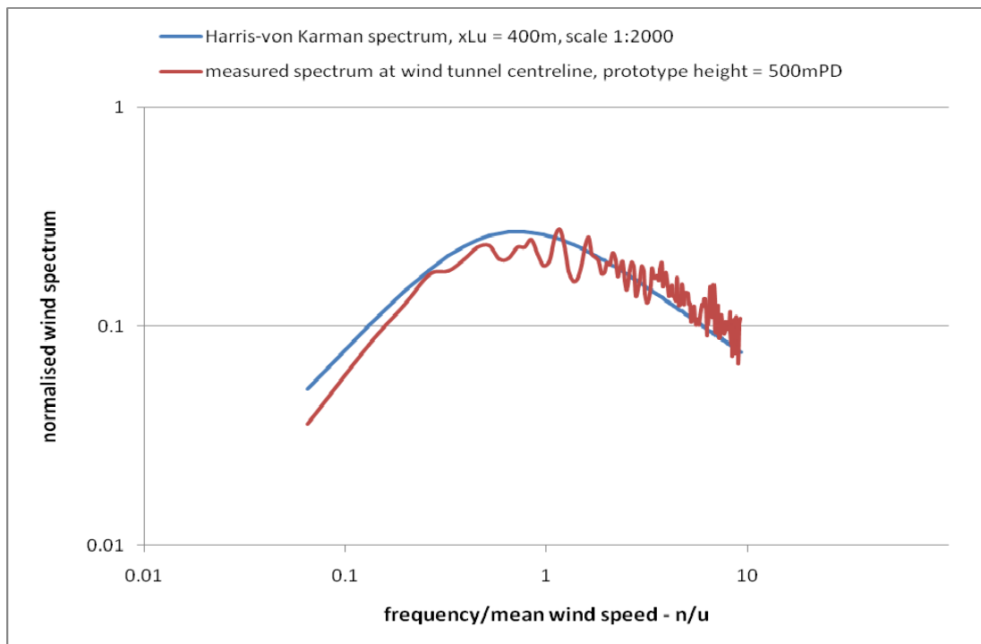
Figure 7: Longitudinal turbulence spectrum of approach wind
