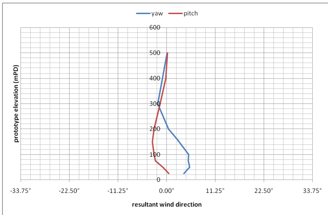
Figure 10b: Mean wind directions for Tseung Kwan O, 45°
