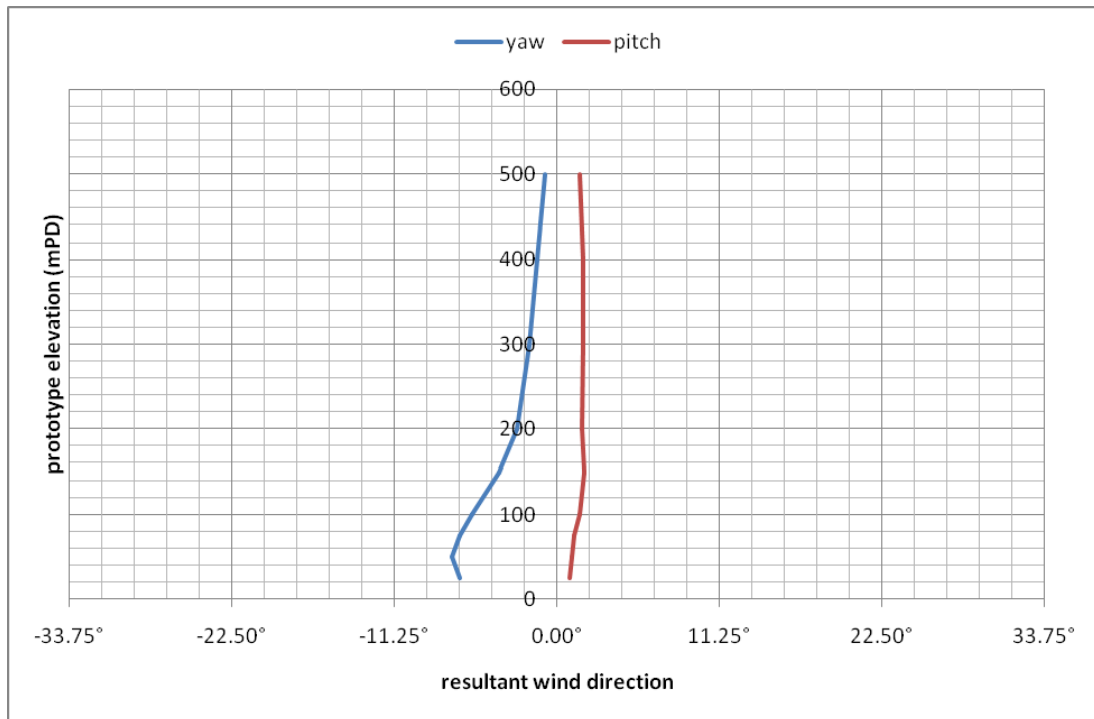
Figure 14b: Mean wind directions for Tseung Kwan O, 135°
