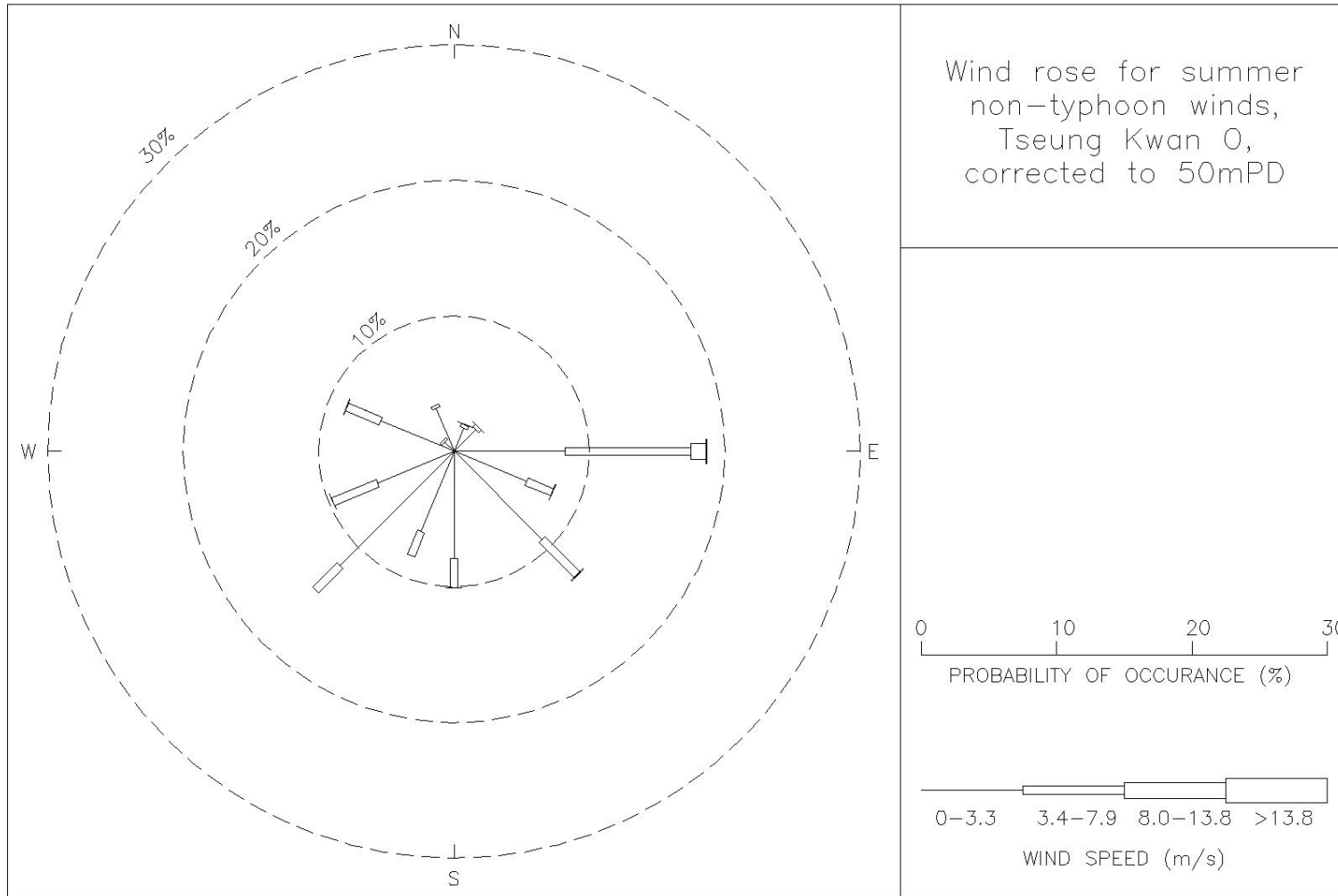
Figure 29: Wind rose for summer, non-typhoon winds for Tseung Kwan O, corrected to 50 mPD
