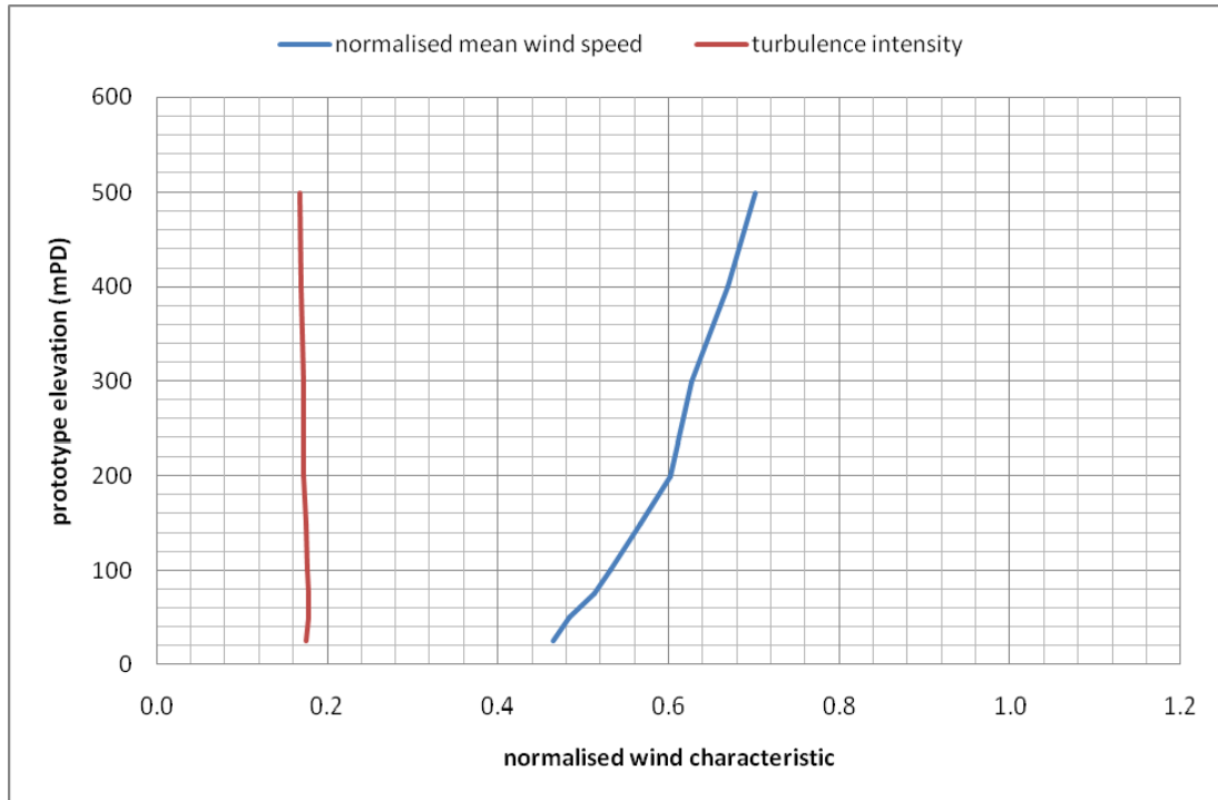
Figure 22a: Wind characteristics for Tseung Kwan O, 315°
