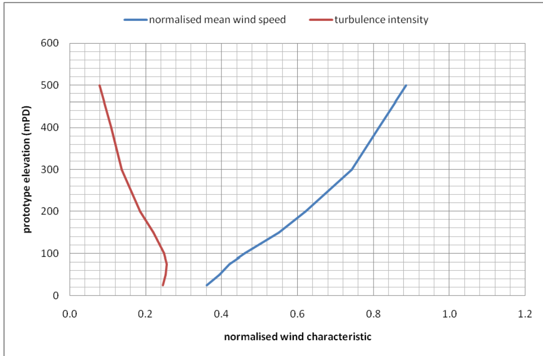
Figure 13a: Wind characteristics for Tseung Kwan O, 112.5°
