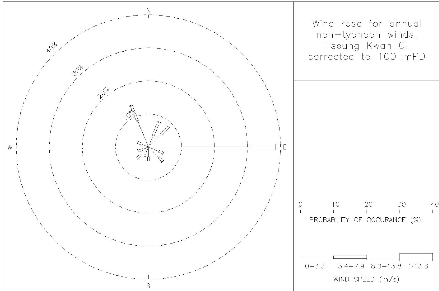
Figure 26: Wind rose for annual, non-typhoon winds for Tseung Kwan O, corrected to 100 mPD
