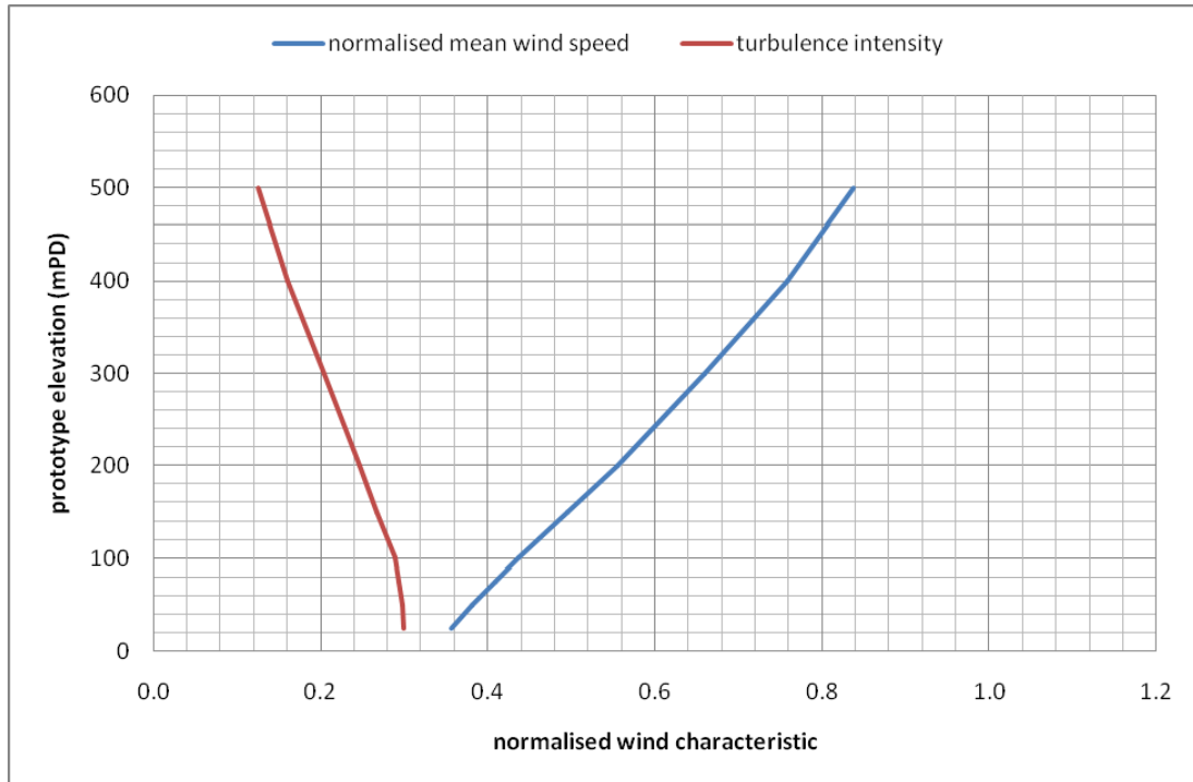
Figure 19a: Wind characteristics for Tseung Kwan O, 247.5°
