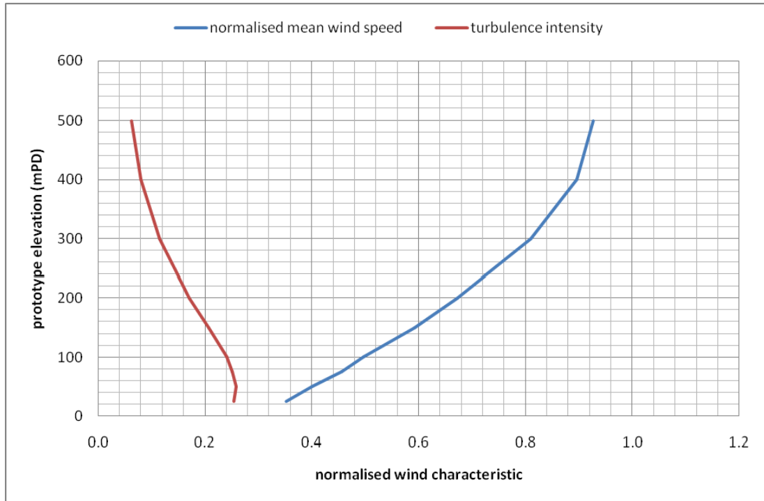
Figure 16a: Wind characteristics for Tseung Kwan O, 180°
