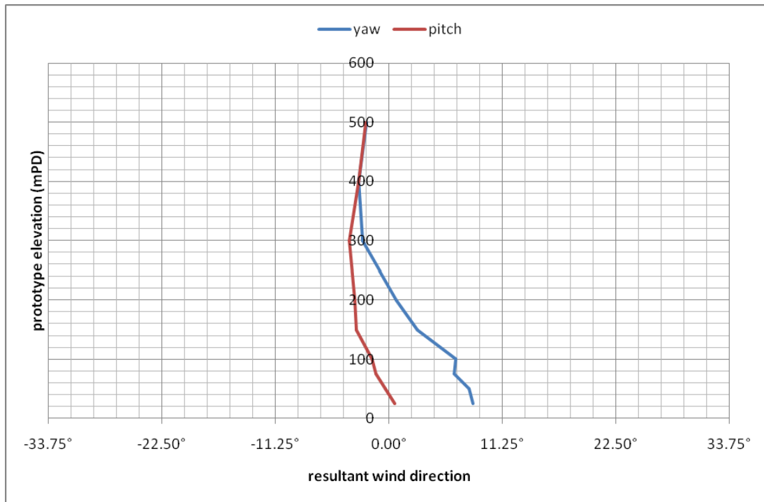
Figure 23b: Mean wind directions for Tseung Kwan O, 337.5°
