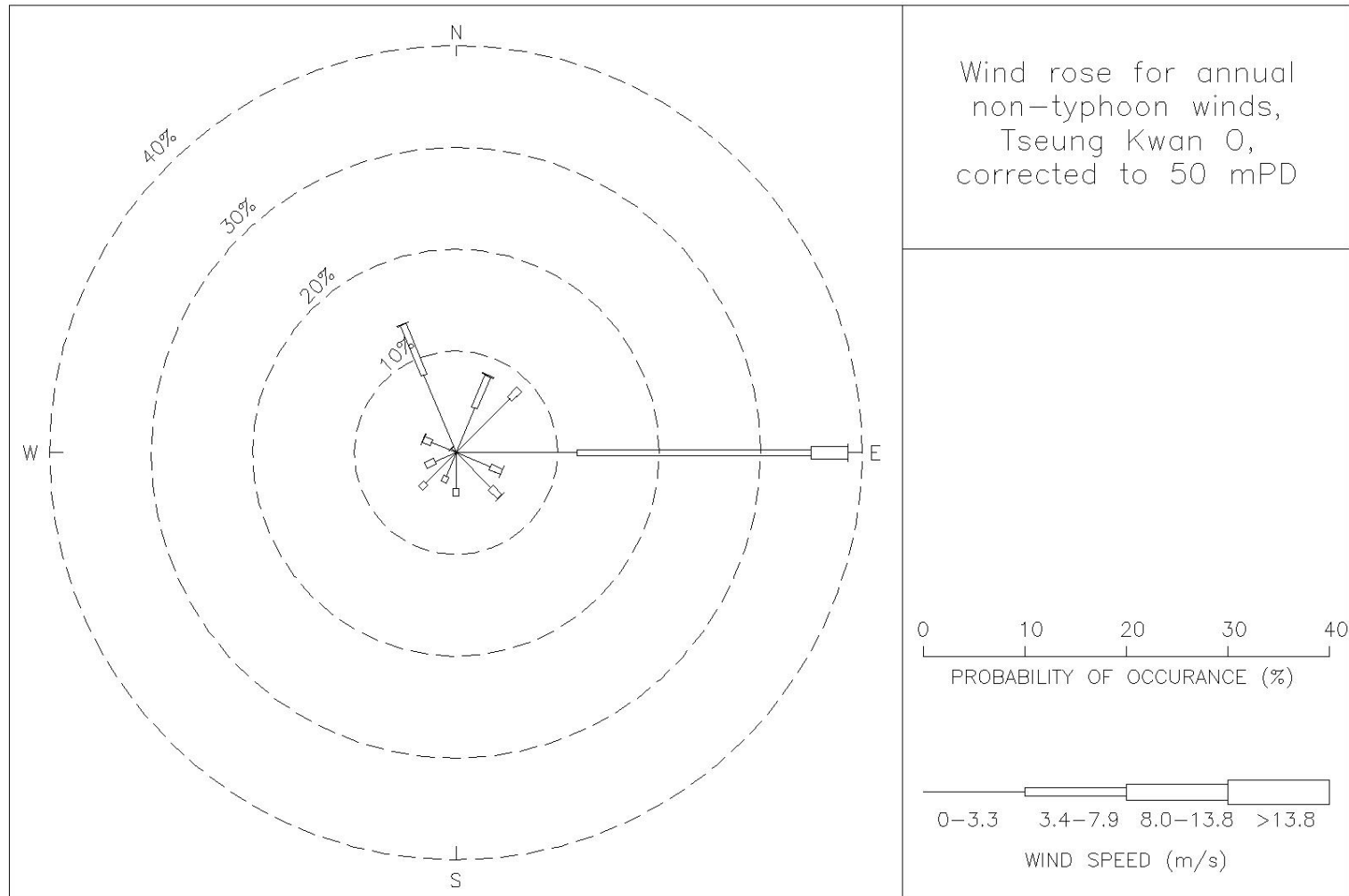
Figure 25: Wind rose for annual, non-typhoon winds for Tseung Kwan O, corrected to 50 mPD
