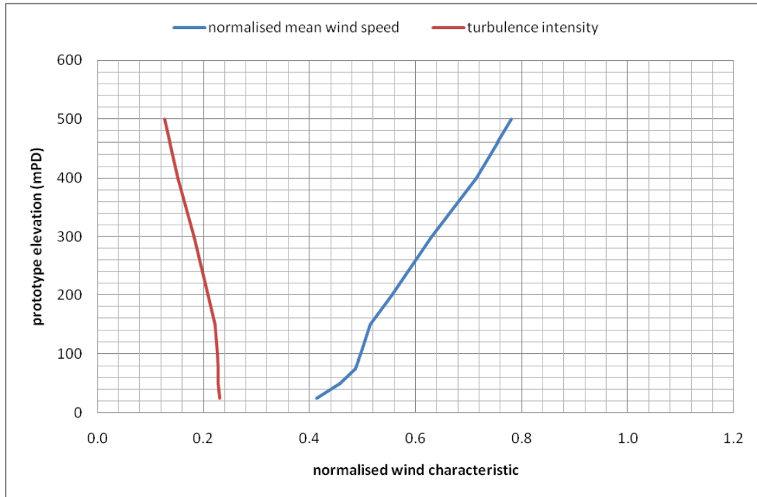
Figure 14a: Wind characteristics for Tseung Kwan O, 135°
