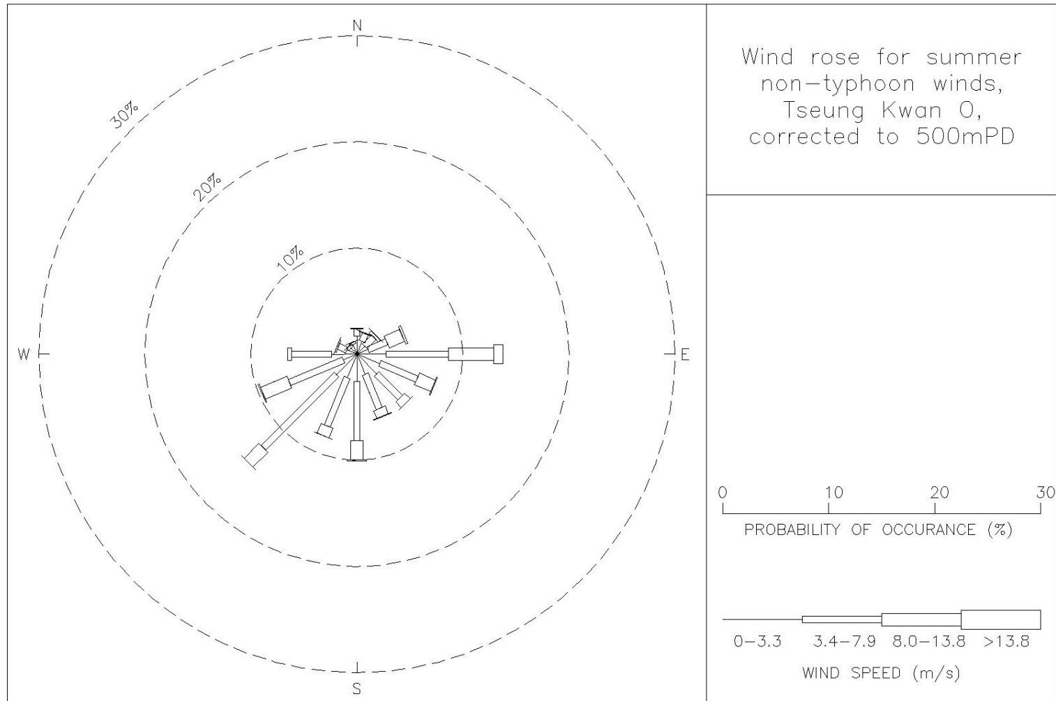
Figure 32: Wind rose for summer, non-typhoon winds for Tseung Kwan O, corrected to 500 mPD
