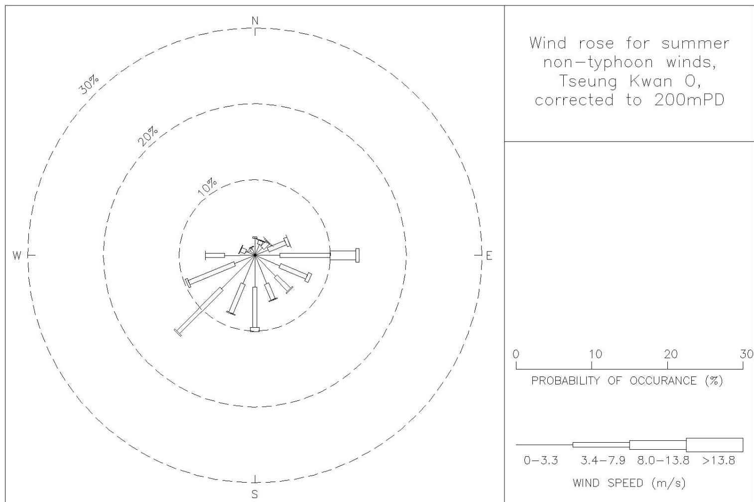
Figure 31: Wind rose for summer, non-typhoon winds for Tseung Kwan O, corrected to 200 mPD
