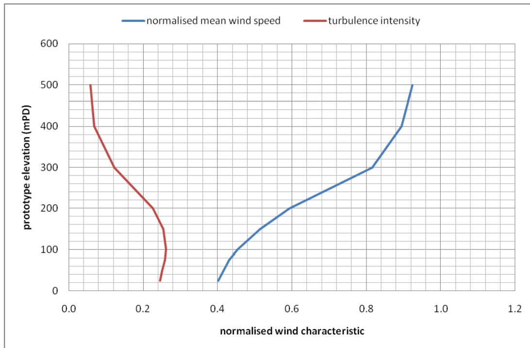
Figure 11a: Wind characteristics for Tseung Kwan O, 67.5°
