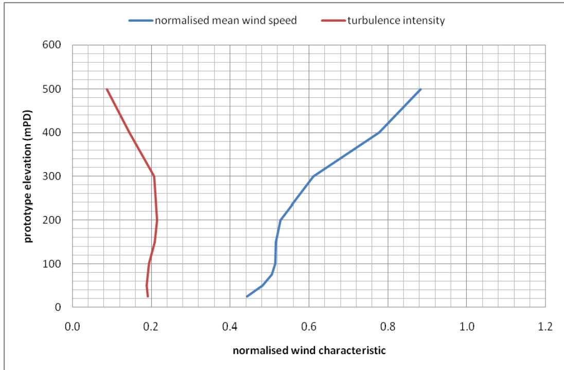
Figure 15a: Wind characteristics for Tseung Kwan O, 157.5°
