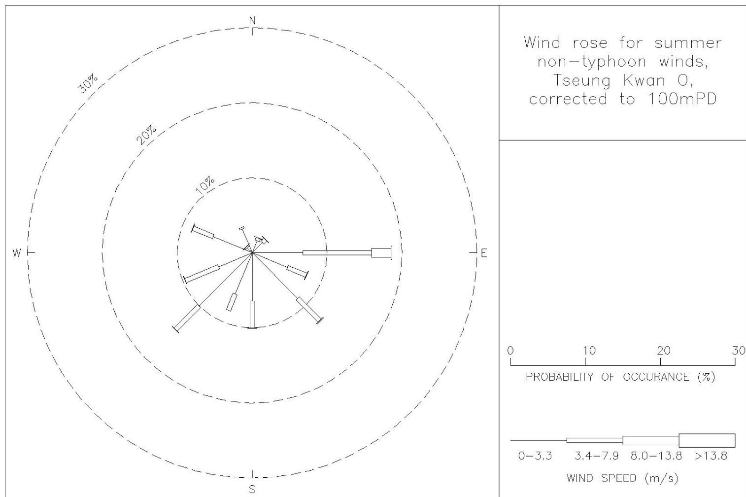
Figure 30: Wind rose for summer, non-typhoon winds for Tseung Kwan O, corrected to 100 mPD
