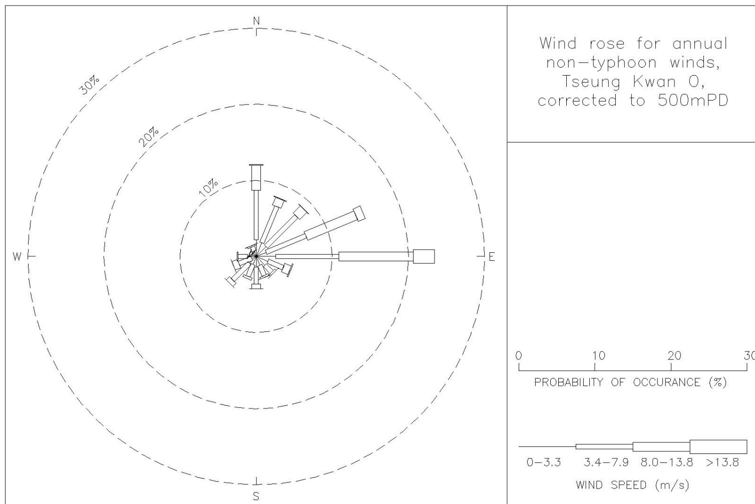
Figure 28: Wind rose for annual, non-typhoon winds for Tseung Kwan O, corrected to 500 mPD
