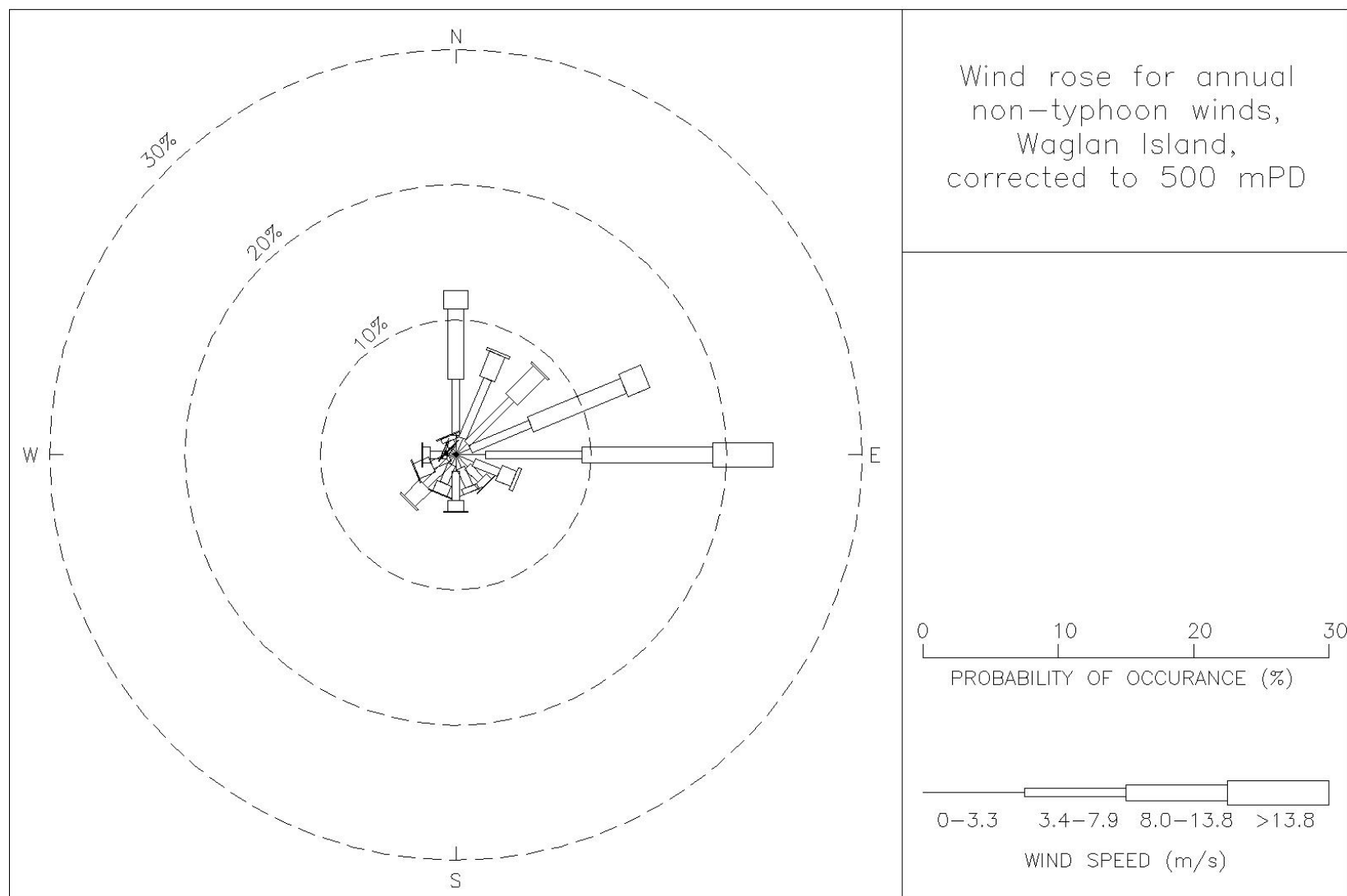
Figure 3: Wind rose for annual non-typhoon winds, Waglan Island, corrected to 500 mPD above open sea, 1953-2006
