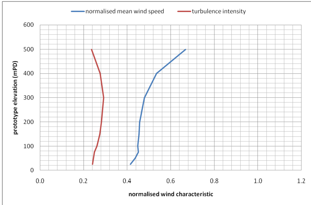
Figure 20a: Wind characteristics for Tseung Kwan O, 270°
