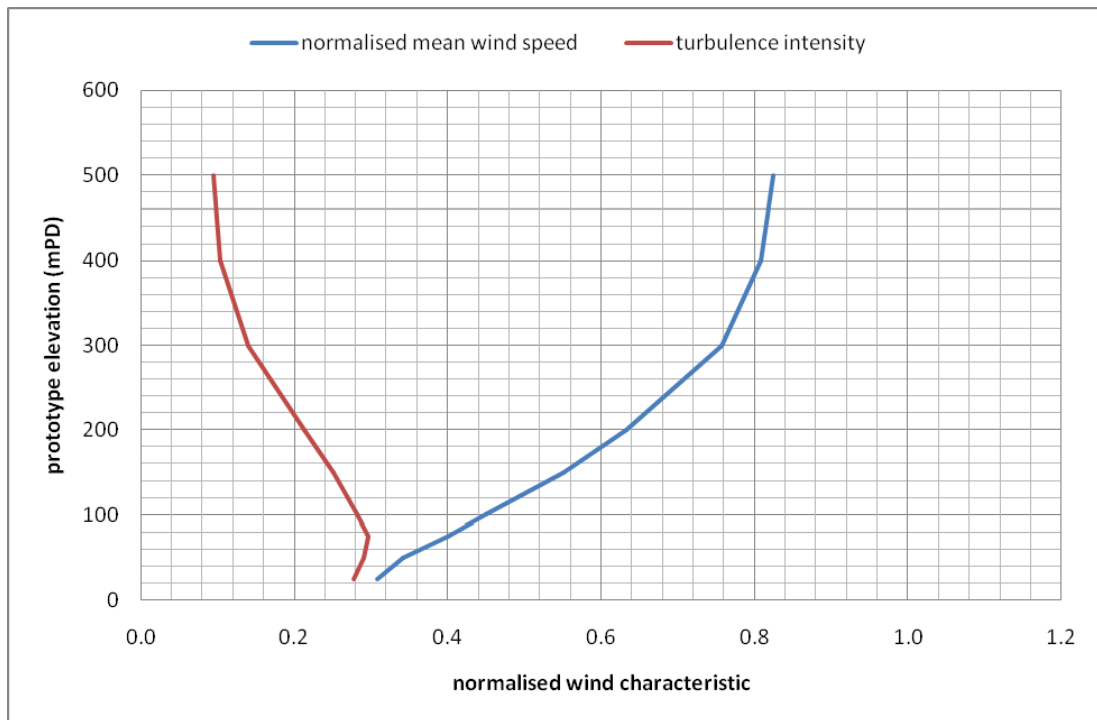
Figure 10a: Wind characteristics for Tseung Kwan O, 45°
