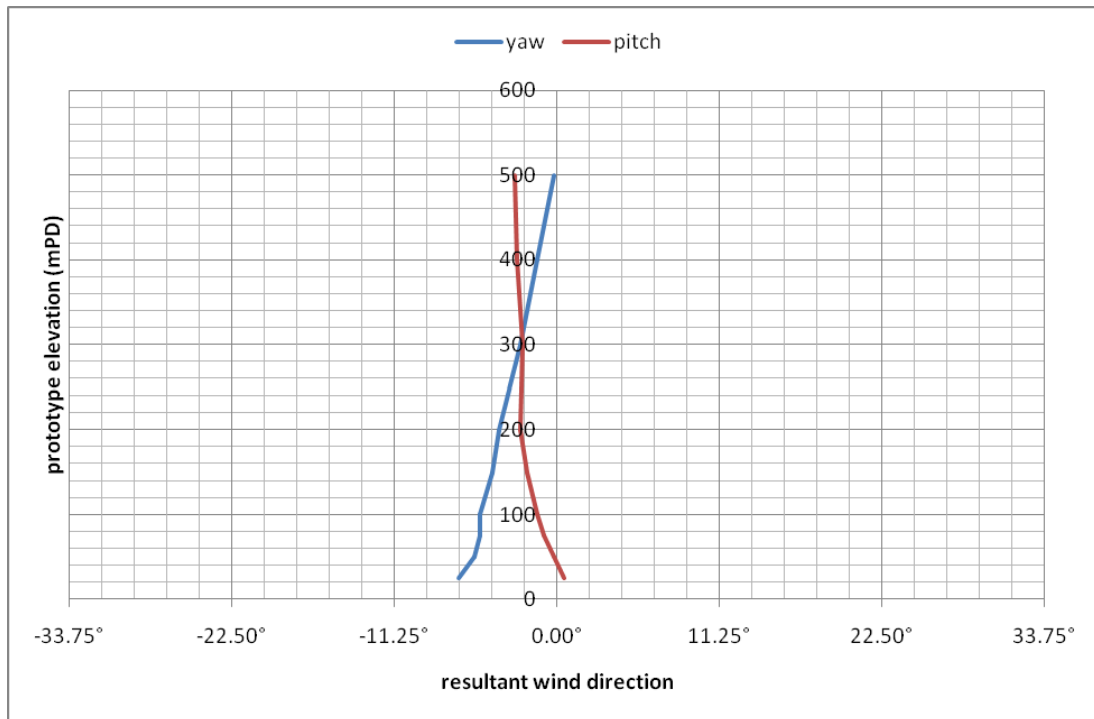
Figure 22b: Mean wind directions for Tseung Kwan O, 315°
