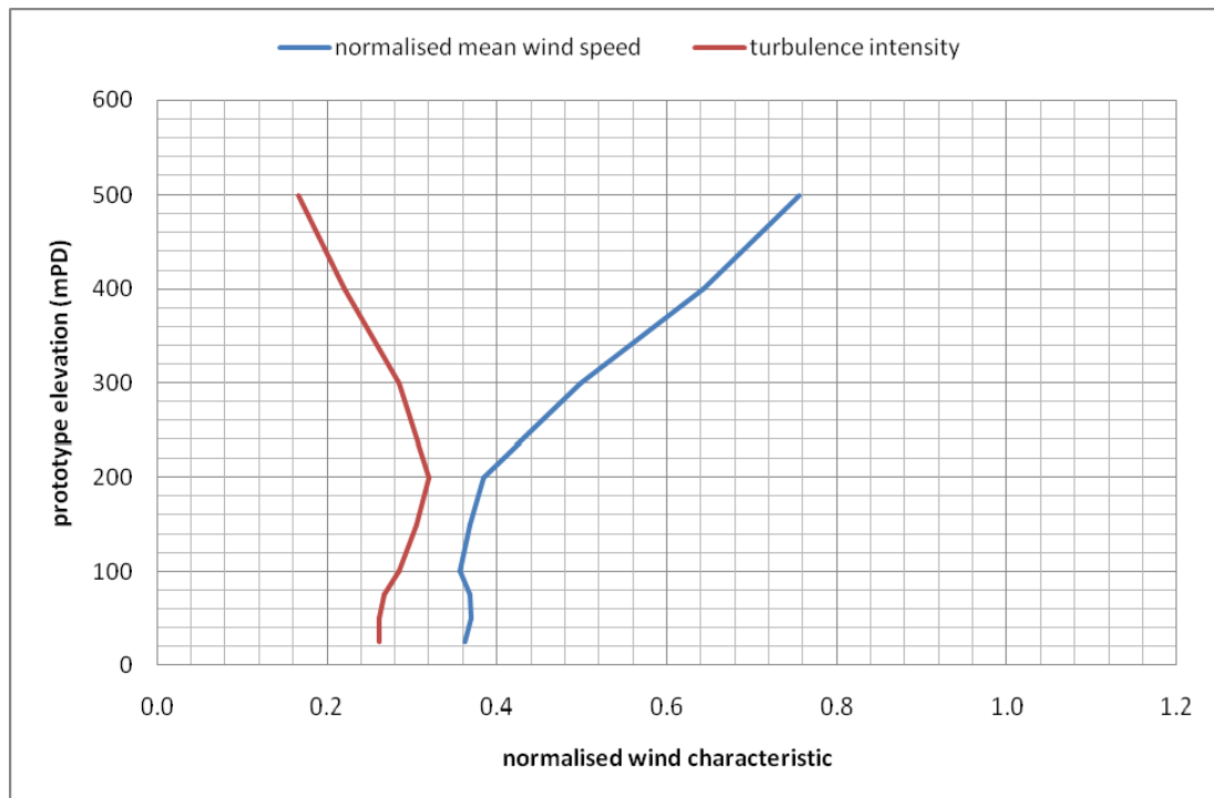
Figure 24a: Wind characteristics for Tseung Kwan O, 360°
