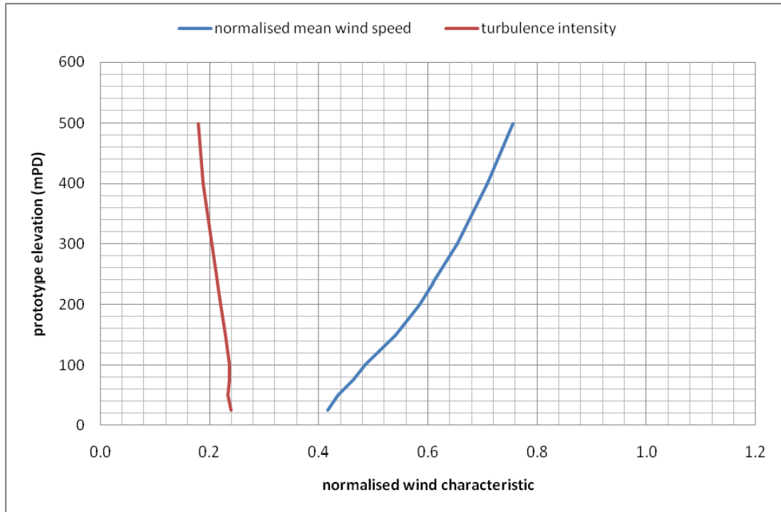
Figure 21a: Wind characteristics for Tseung Kwan O, 292.5°
