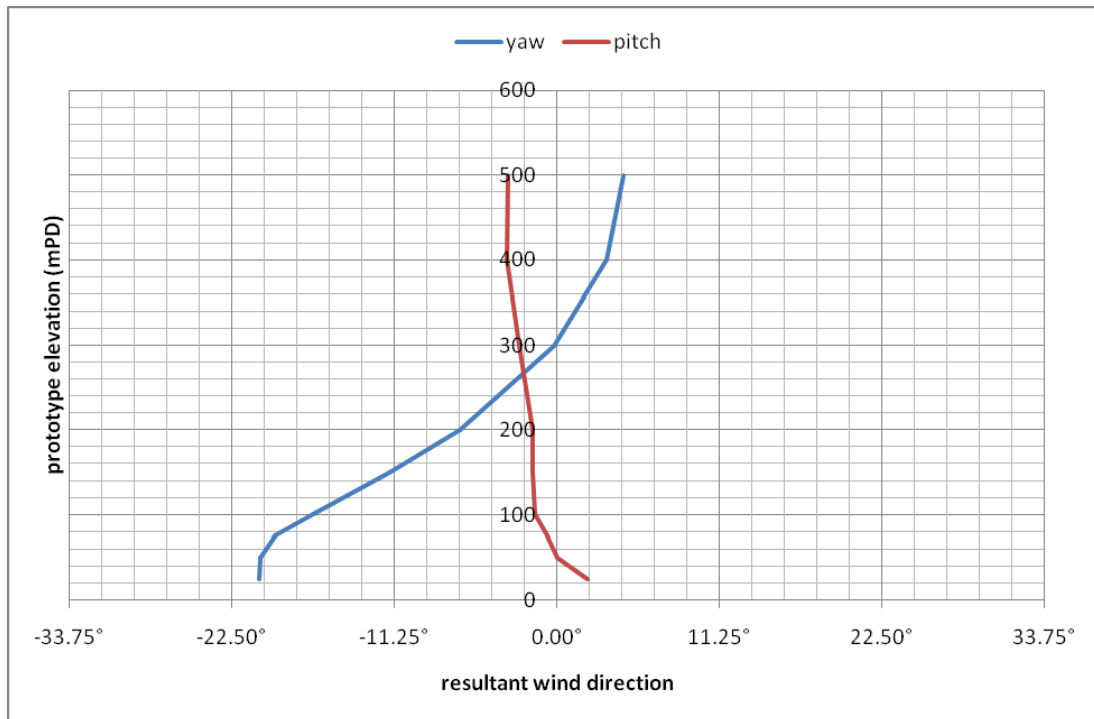
Figure 20b: Mean wind directions for Tseung Kwan O, 270°
