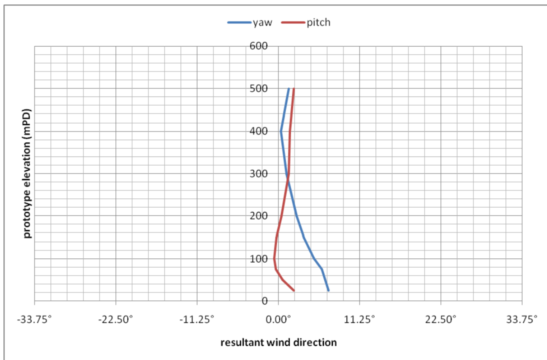
Figure 18b: Mean wind directions for Tseung Kwan O, 225°
