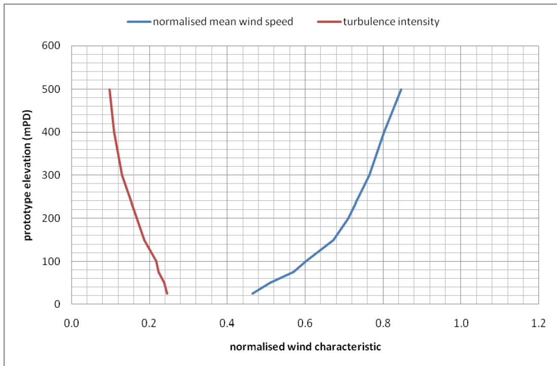
Figure 9a: Wind characteristics for Tseung Kwan O, 22.5°
