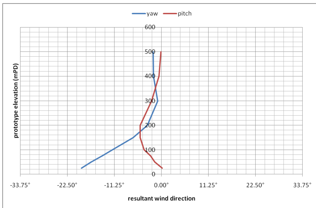
Figure 11b: Mean wind directions for Tseung Kwan O, 67.5°
