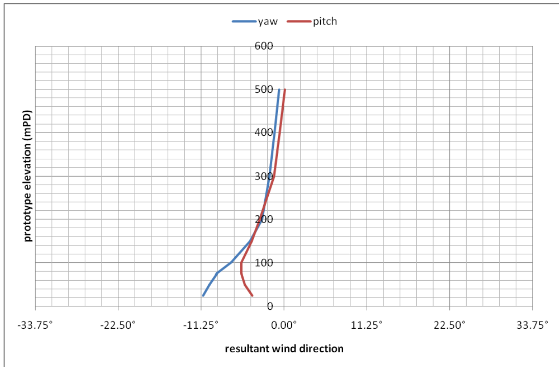
Figure 12b: Mean wind directions for Tseung Kwan O, 90°
