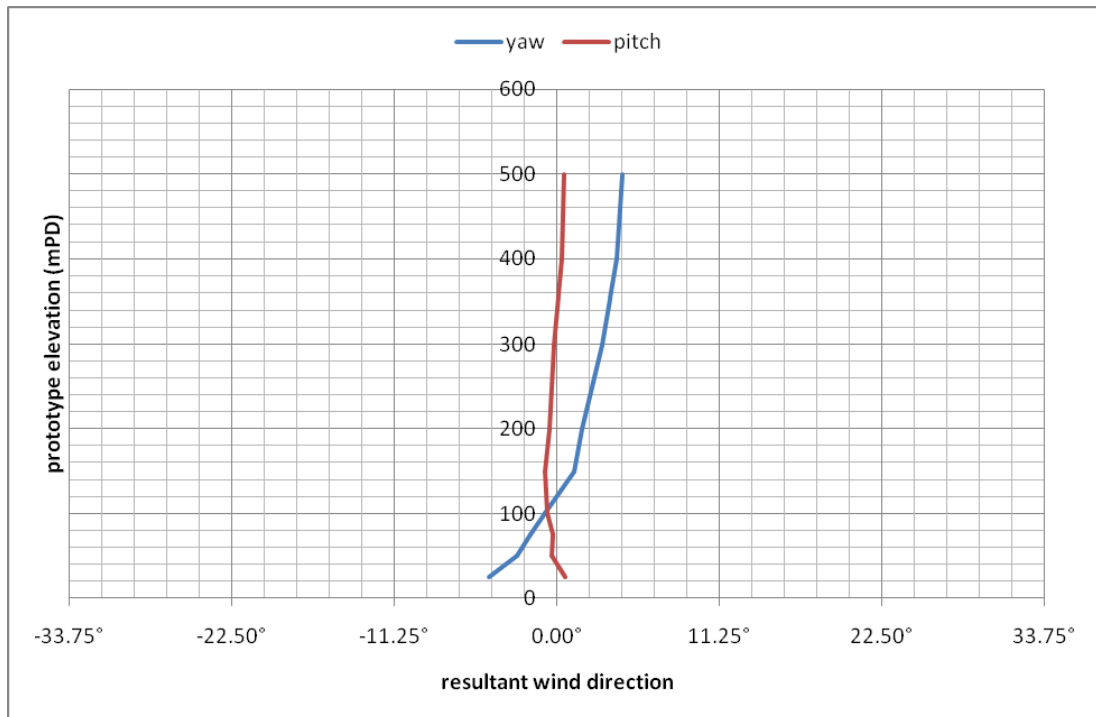
Figure 13b: Mean wind directions for Tseung Kwan O, 112.5°
