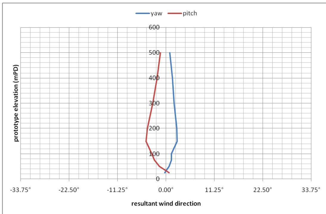
Figure 19b: Mean wind directions for Tseung Kwan O, 247.5°
