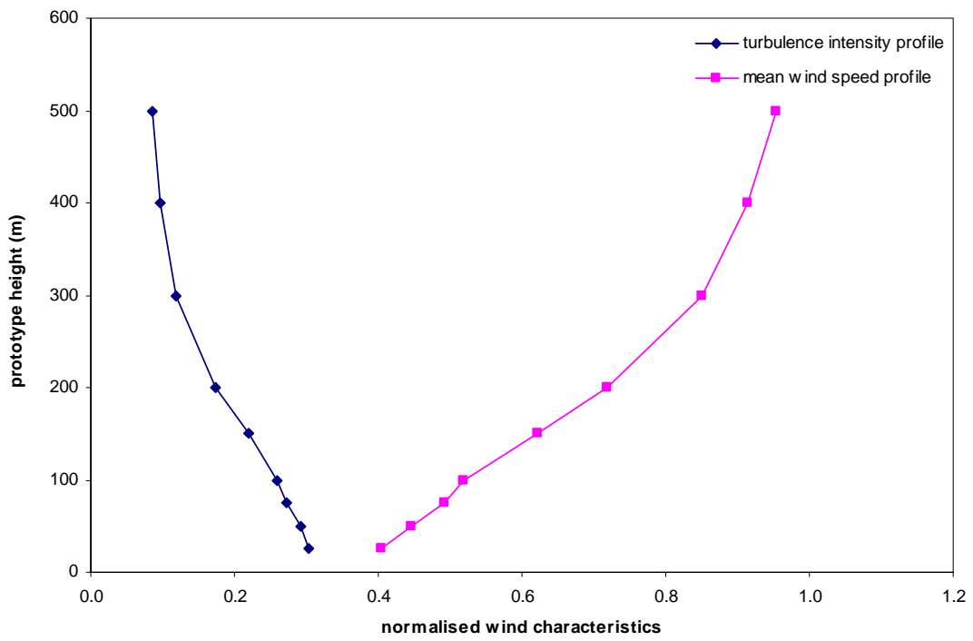
Figure 10a: Wind characteristics, Tsim Sha Tsui, 67.5°
