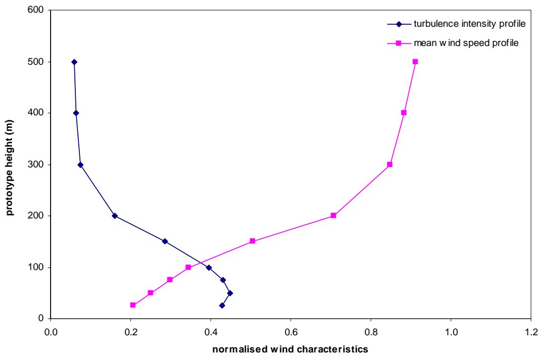
Figure 18a: Wind characteristics, Tsim Sha Tsui, 247.5°
