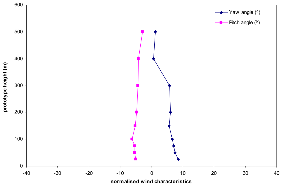
Figure 9b: Mean wind direction, Tsim Sha Tsui, 45°
