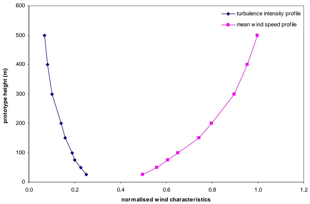
Figure 14a: Wind characteristics, Tsim Sha Tsui, 157.5°
