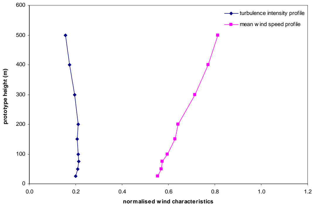
Figure 13a: Wind characteristics, Tsim Sha Tsui, 135°
