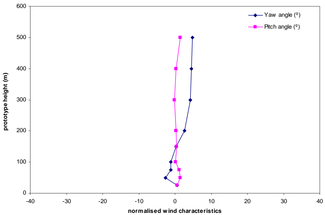
Figure 11b: Mean wind direction, Tsim Sha Tsui, 90°
