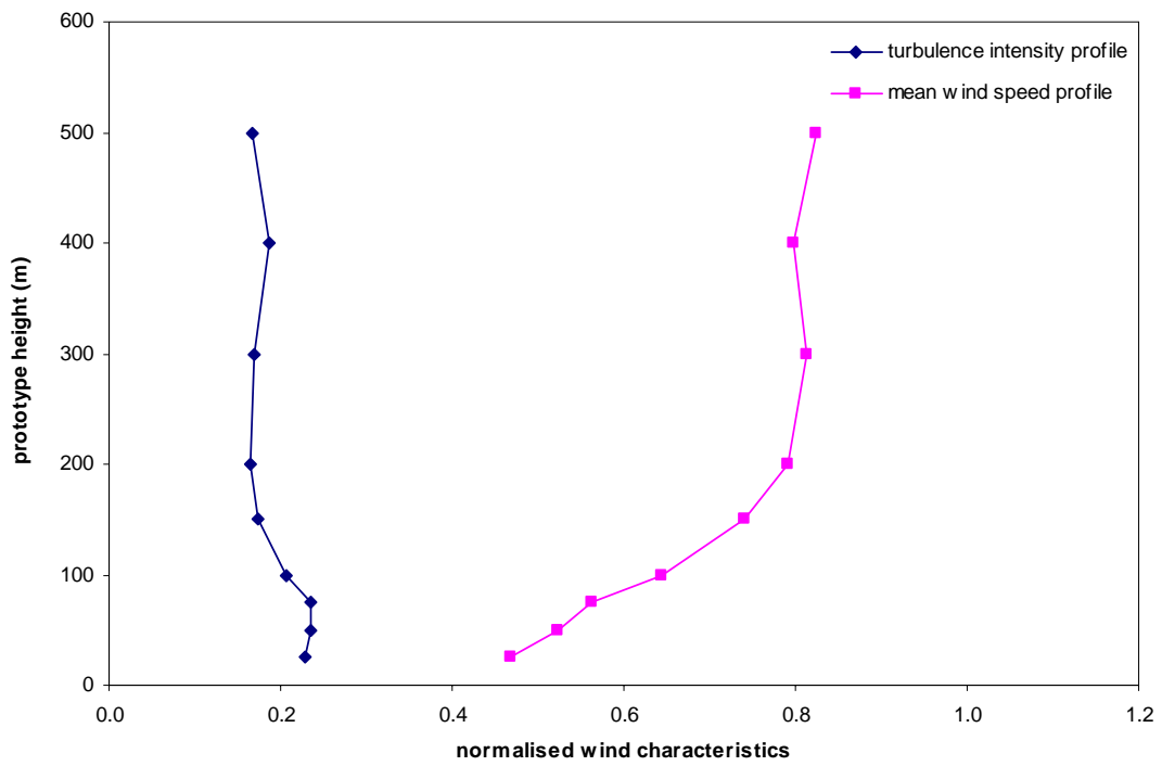
Figure 17a: Wind characteristics, Tsim Sha Tsui, 225°
