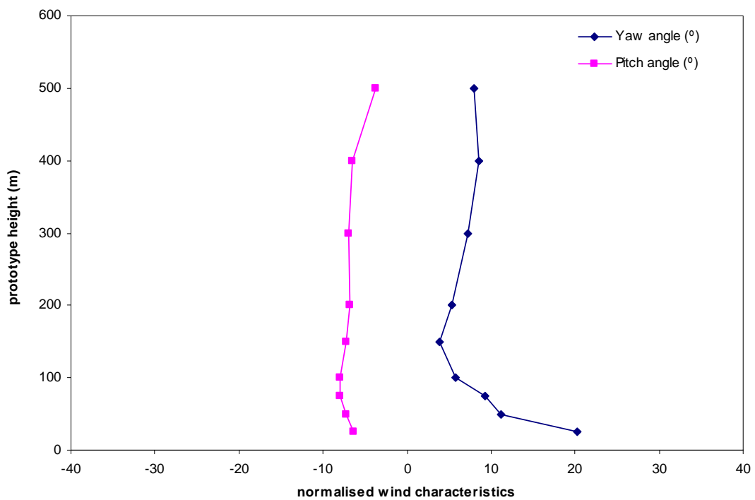
Figure 17b: Mean wind direction, Tsim Sha Tsui, 225°
