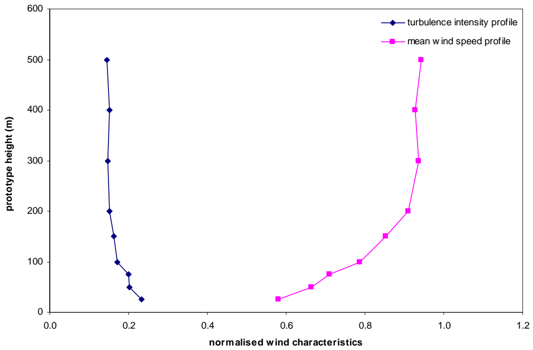
Figure 9a: Wind characteristics, Tsim Sha Tsui, 45°
