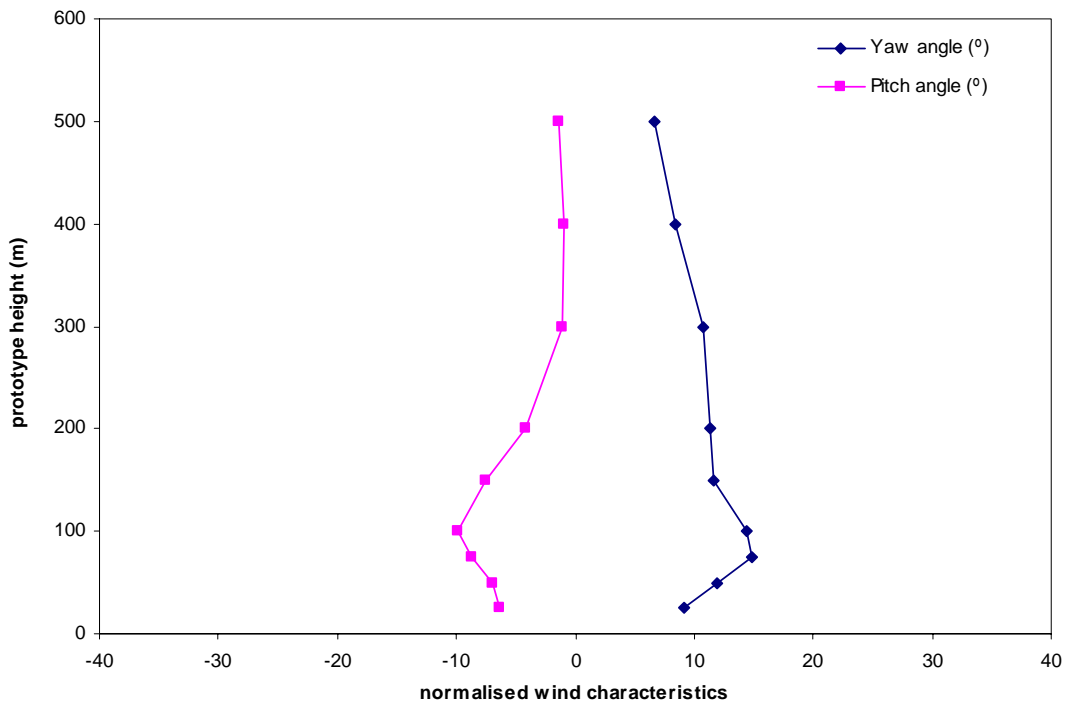
Figure 19b: Mean wind direction, Tsim Sha Tsui, 270°
