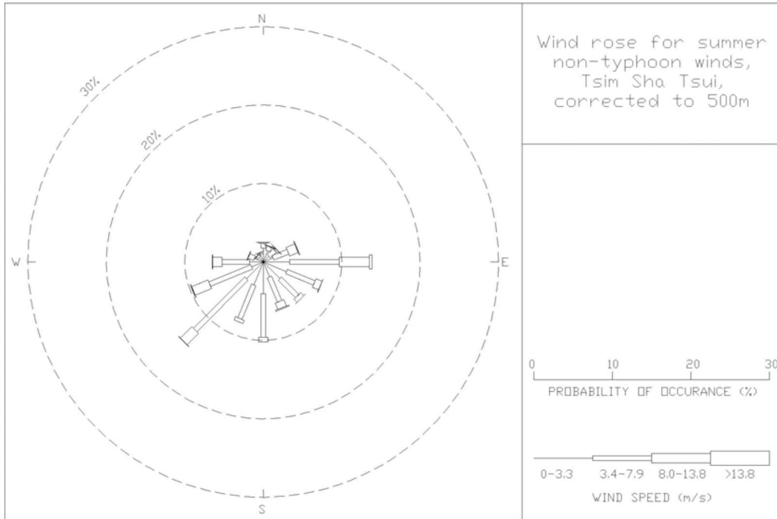
Figure 31: Wind rose for summer, non-typhoon winds for Tsim Sha Tsui, corrected to 500 m
