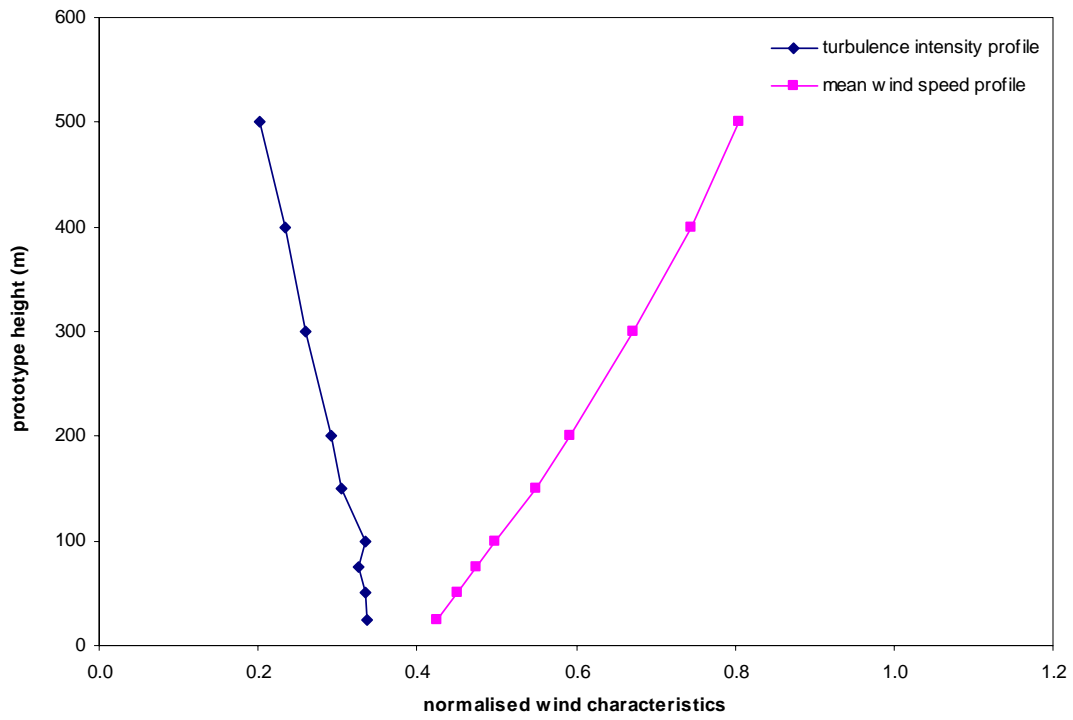
Figure 23a: Wind characteristics, Tsim Sha Tsui, 360°
