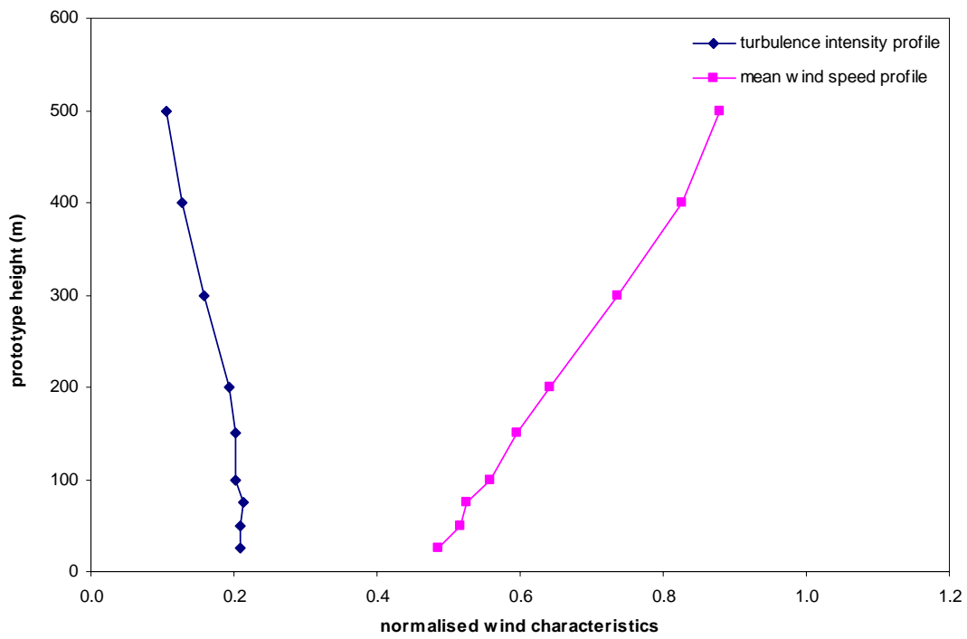
Figure 12a: Wind characteristics, Tsim Sha Tsui, 112.5°
