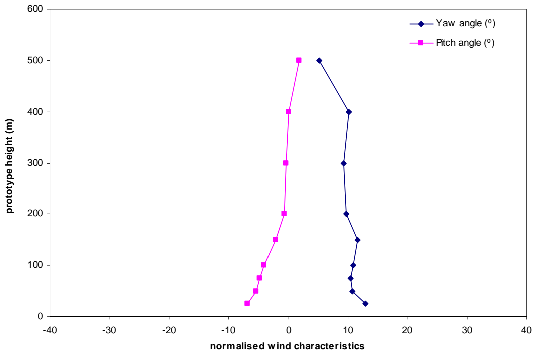
Figure 21b: Mean wind direction, Tsim Sha Tsui, 315°
