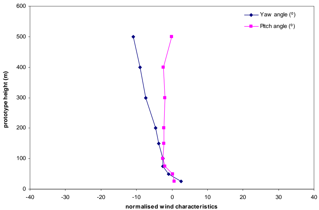
Figure 10b: Mean wind direction, Tsim Sha Tsui, 67.5°
