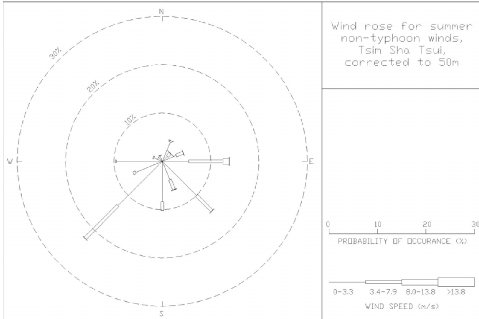
Figure 28: Wind rose for summer, non-typhoon winds for Tsim Sha Tsui, corrected to 50 m
