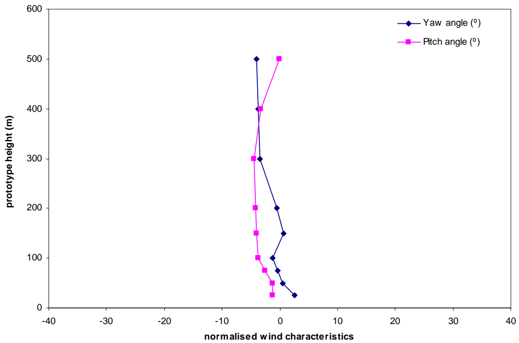
Figure 13b: Mean wind direction, Tsim Sha Tsui, 135°
