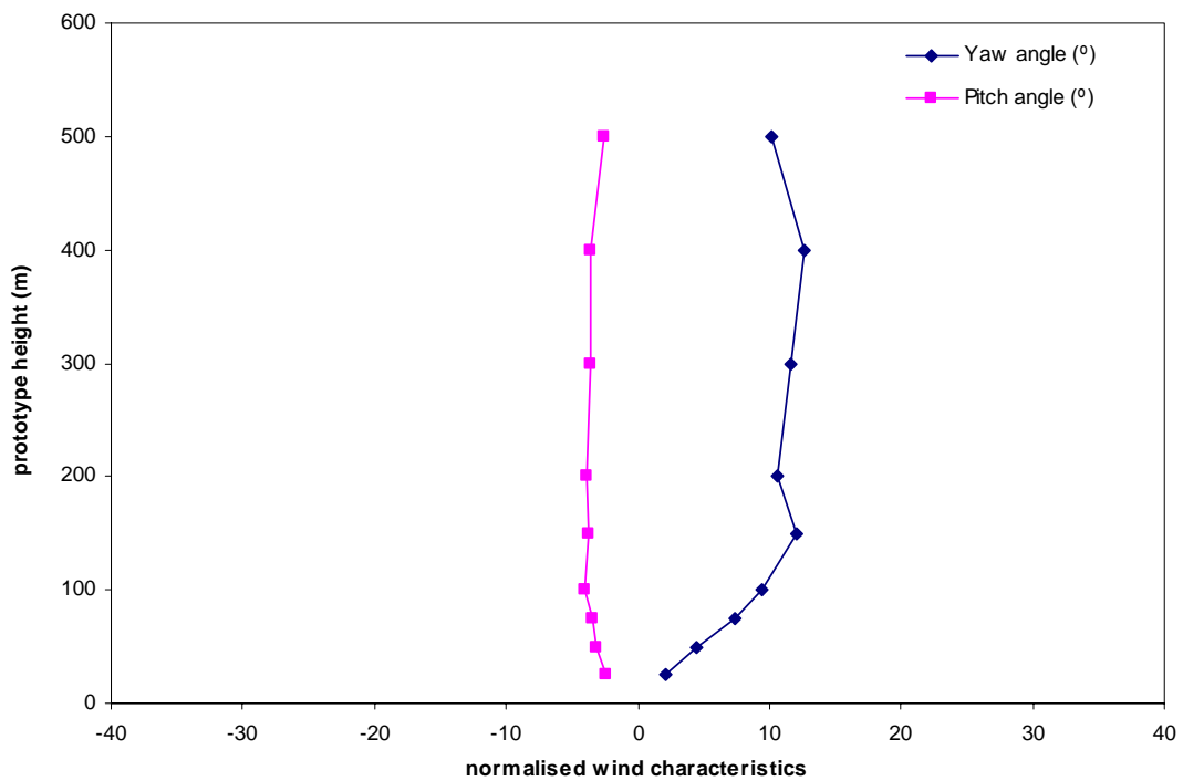
Figure 22b: Mean wind direction, Tsim Sha Tsui, 337.5°
