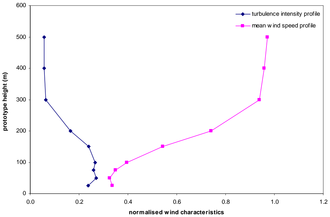
Figure 19a: Wind characteristics, Tsim Sha Tsui, 270°
