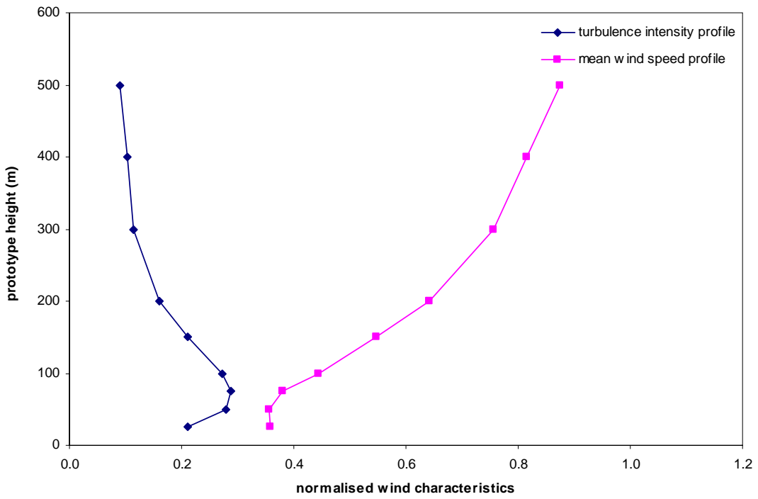
Figure 21a: Wind characteristics, Tsim Sha Tsui, 315°
