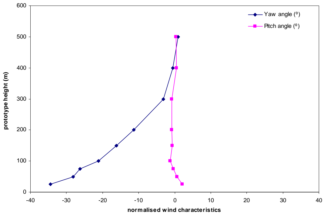
Figure 16b: Mean wind direction, Tsim Sha Tsui, 202.5°
