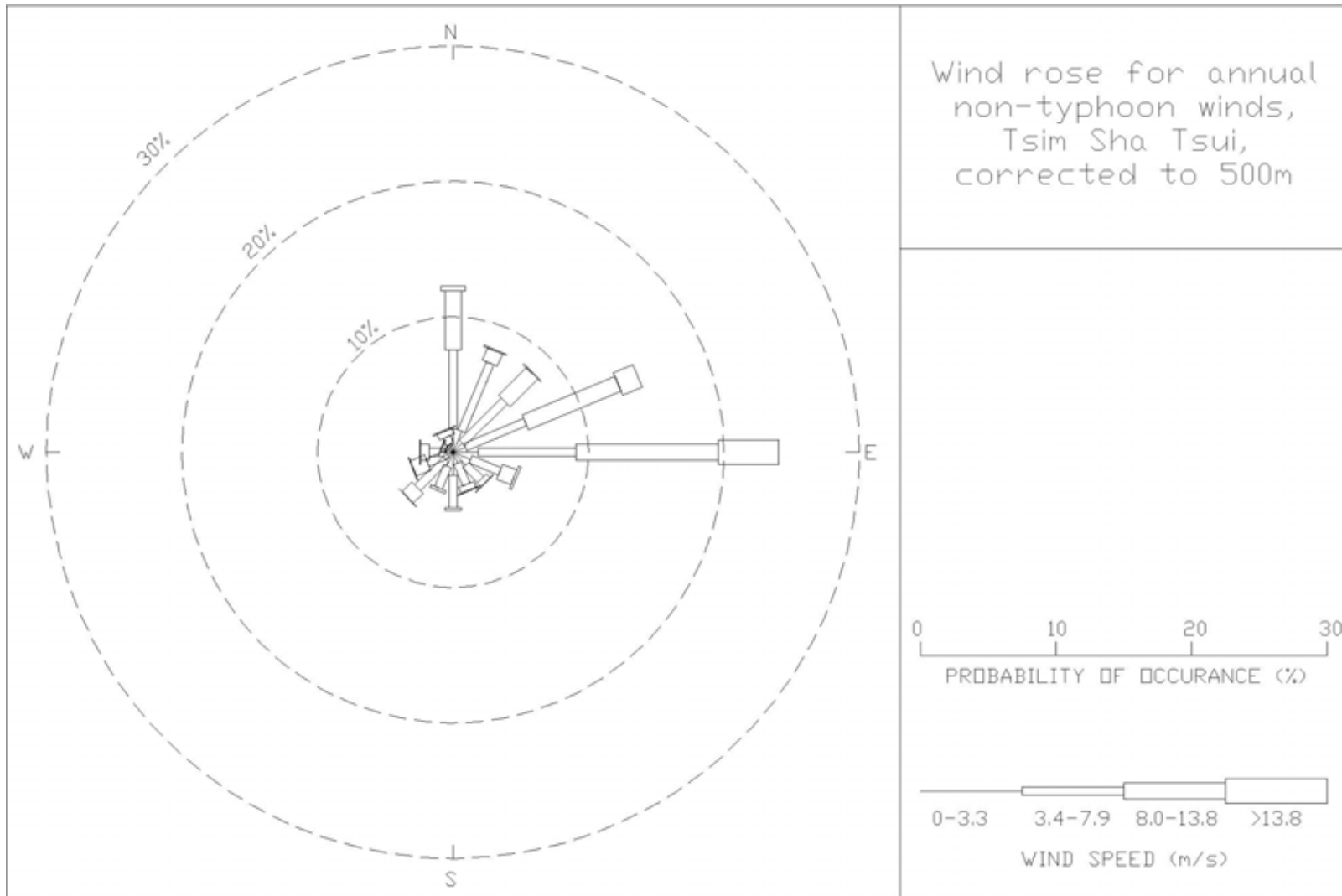
Figure 27: Wind rose for annual, non-typhoon winds for Tsim Sha Tsui, corrected to 500 m
