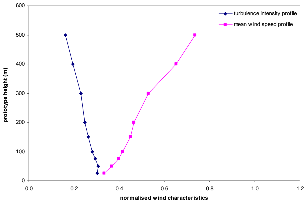
Figure 20a: Wind characteristics, Tsim Sha Tsui, 292.5°
