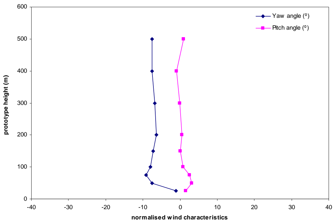
Figure 8b: Mean wind direction, Tsim Sha Tsui, 22.5°
