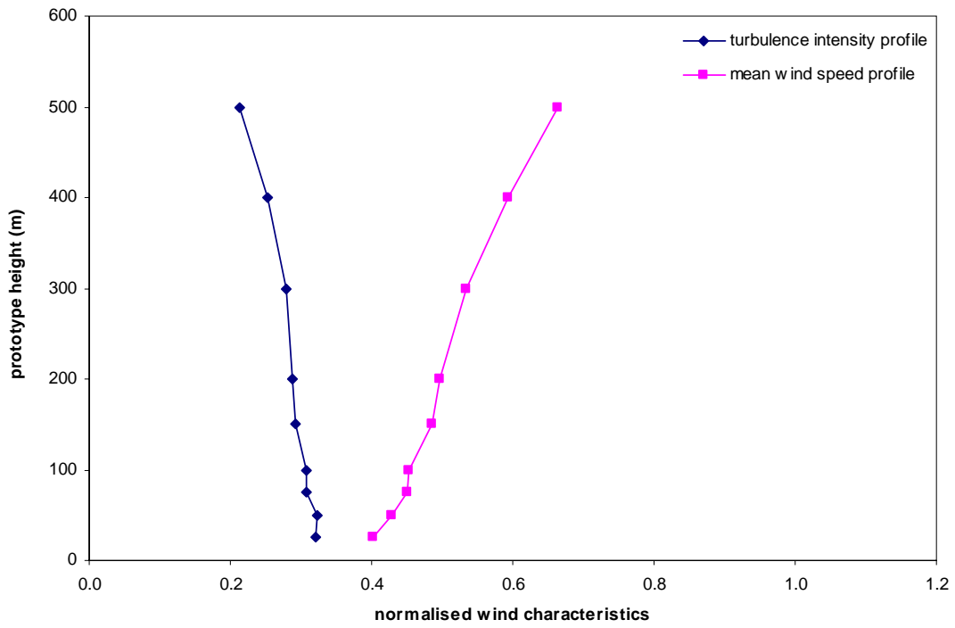
Figure 16a: Wind characteristics, Tsim Sha Tsui, 202.5°
