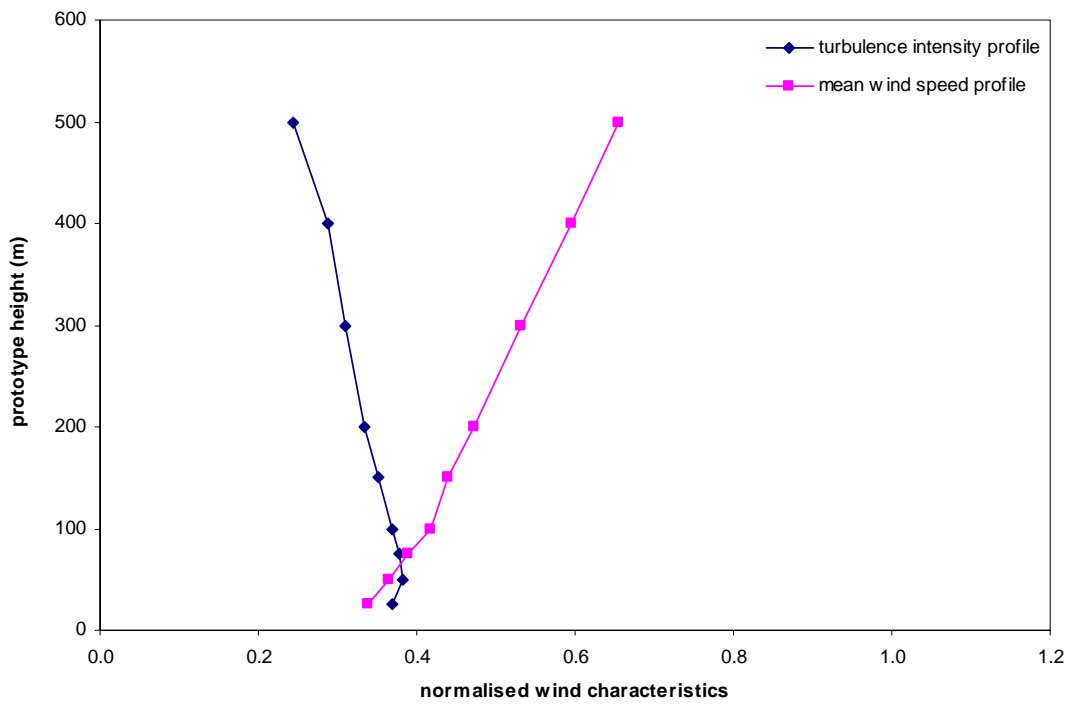
Figure 15a: Wind characteristics, Tsim Sha Tsui, 180°
