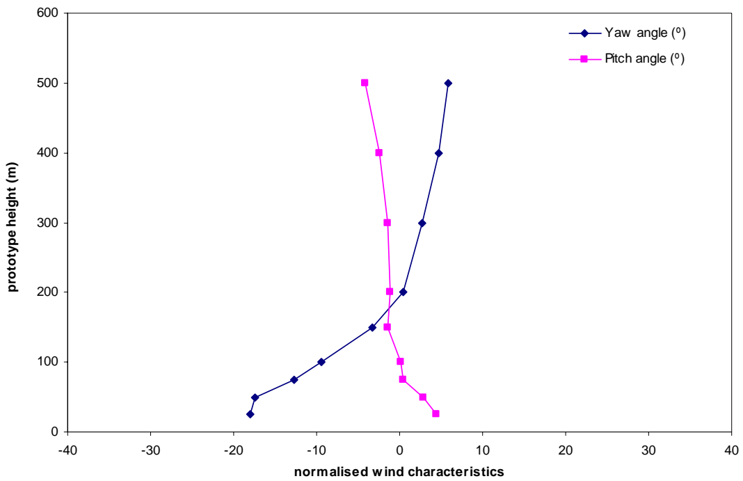
Figure 23b: Mean wind direction, Tsim Sha Tsui, 360°
