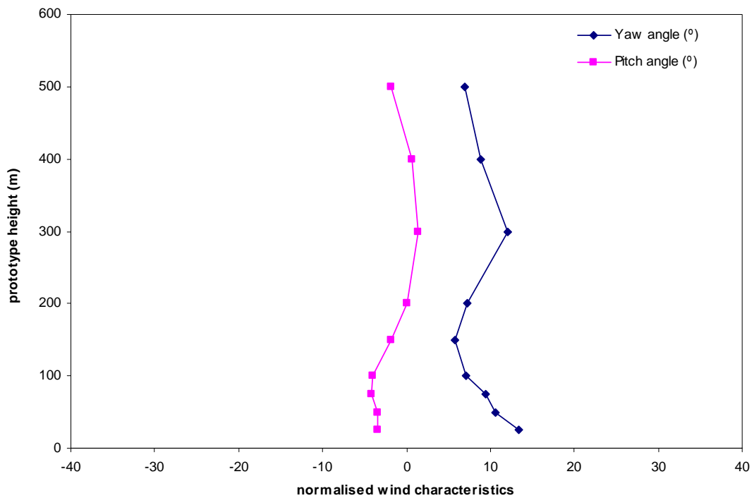
Figure 20b: Mean wind direction, Tsim Sha Tsui, 292.5°
