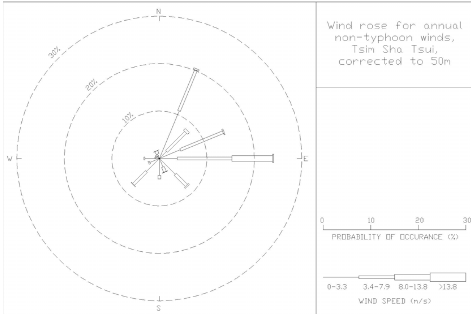
Figure 24: Wind rose for annual, non-typhoon winds for Tsim Sha Tsui, corrected to 50 m
