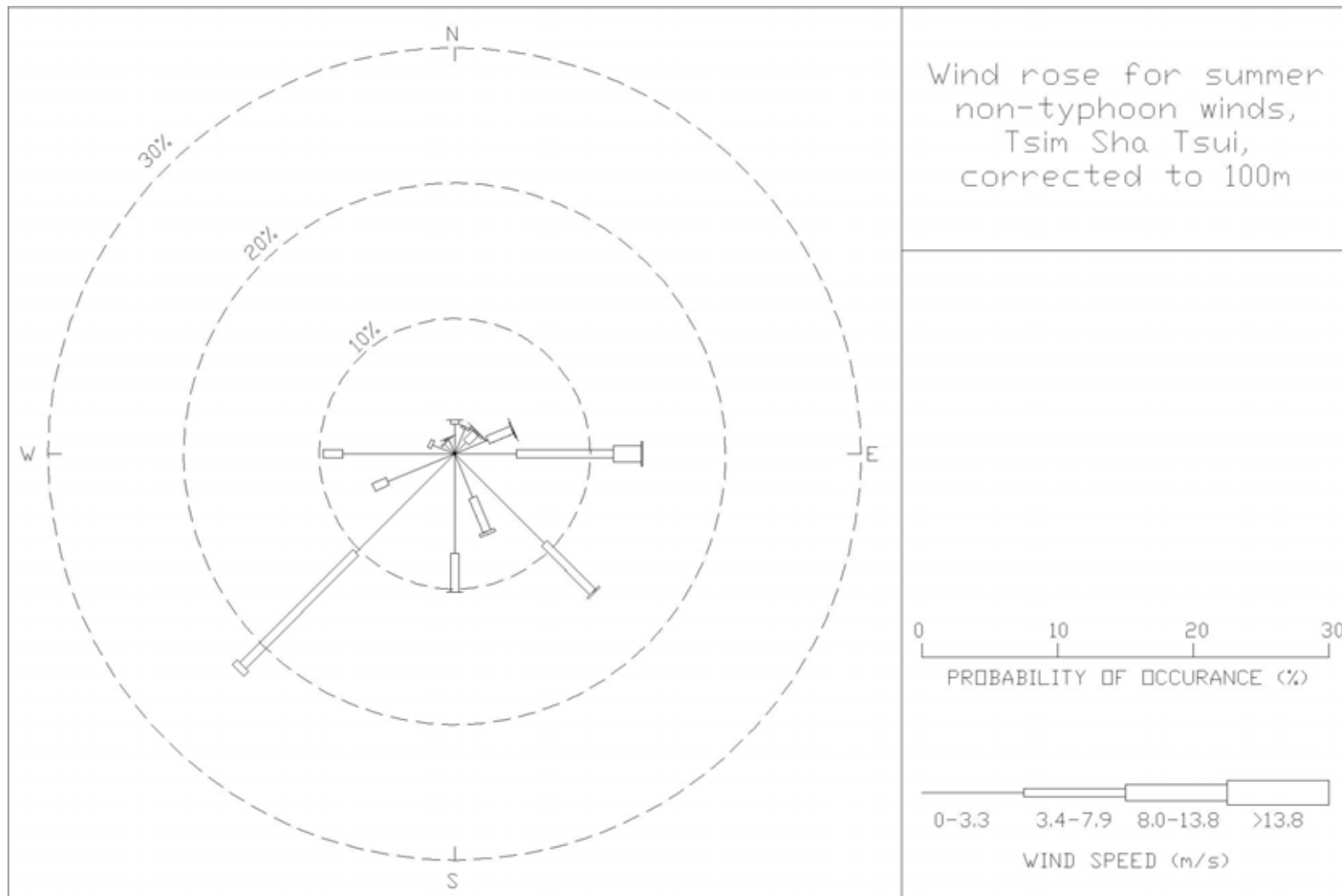
Figure 29: Wind rose for summer, non-typhoon winds for Tsim Sha Tsui, corrected to 100 m
