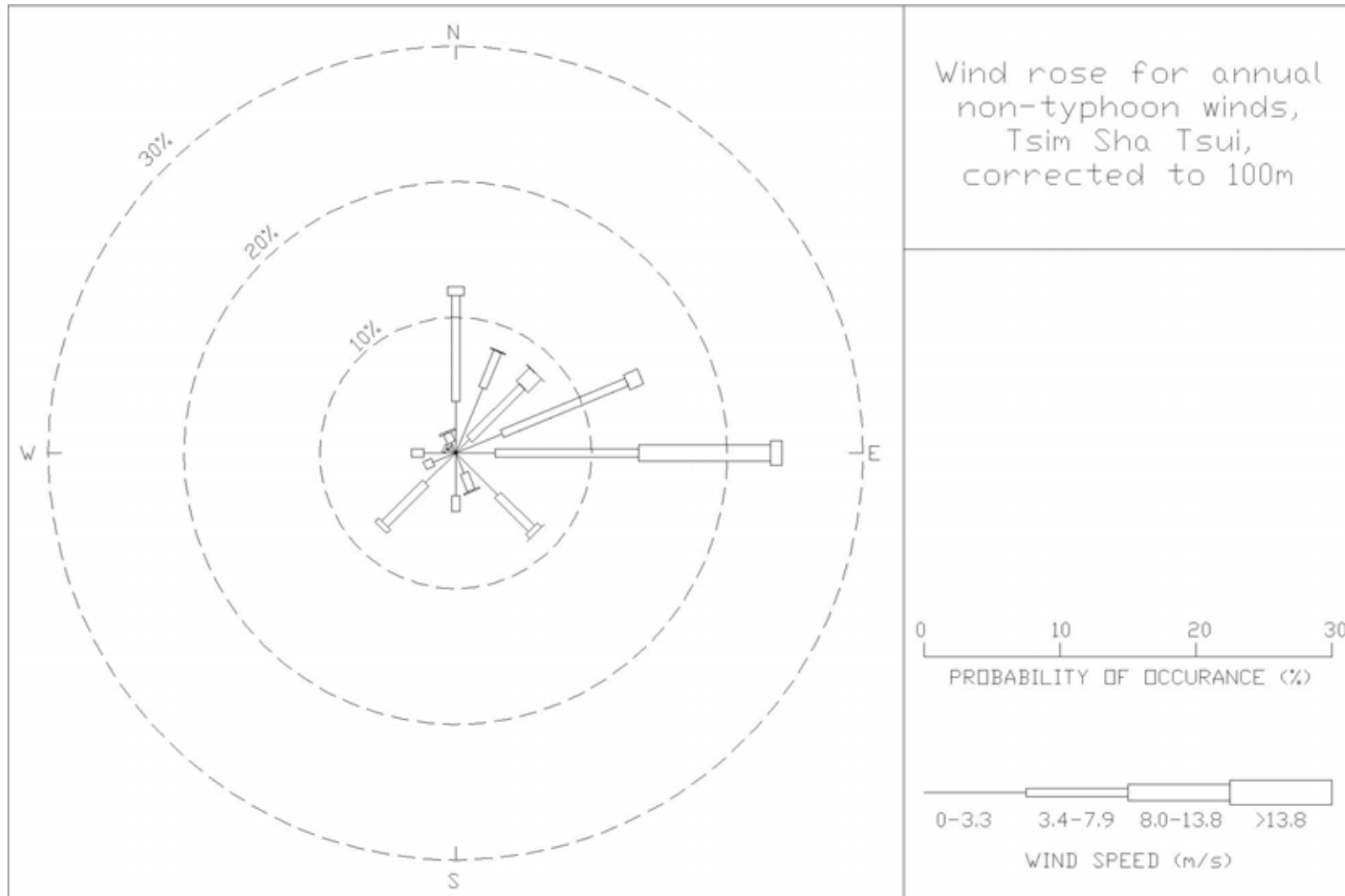
Figure 25: Wind rose for annual, non-typhoon winds for Tsim Sha Tsui, corrected to 100 m
