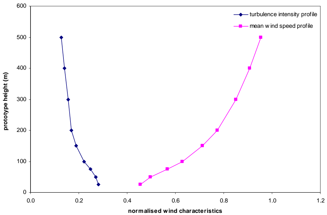
Figure 22a: Wind characteristics, Tsim Sha Tsui, 337.5°
