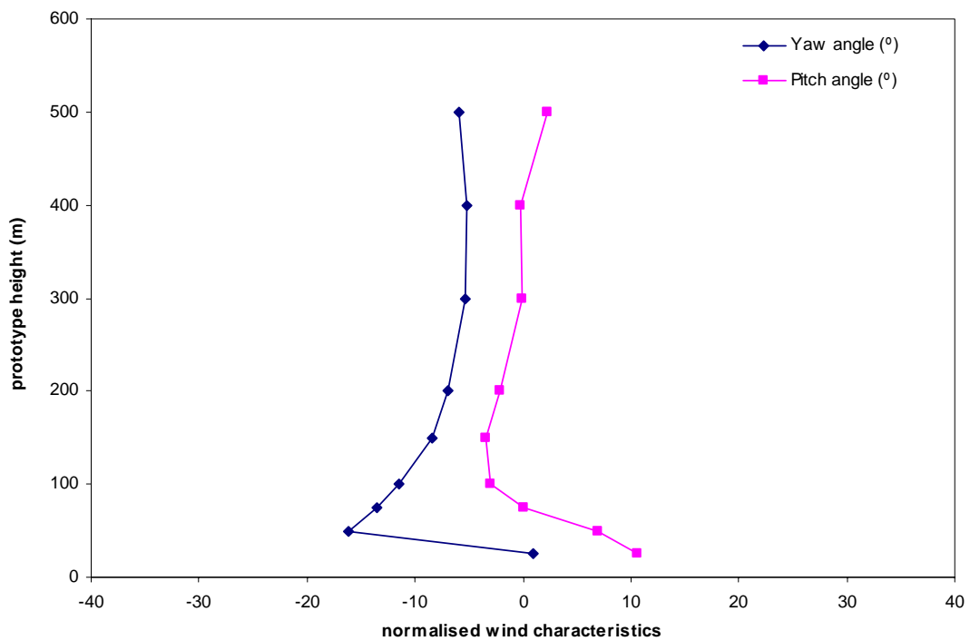
Figure 18b: Mean wind direction, Tsim Sha Tsui, 247.5°
