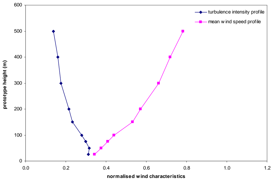
Figure 8a: Wind characteristics, Tsim Sha Tsui, 22.5°
