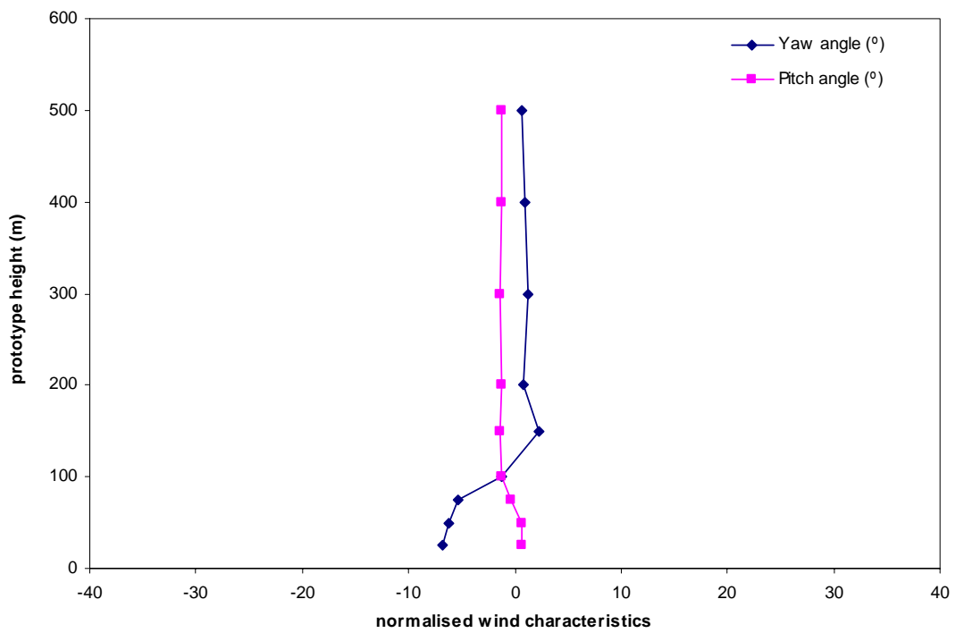
Figure 14b: Mean wind direction, Tsim Sha Tsui, 157.5°
