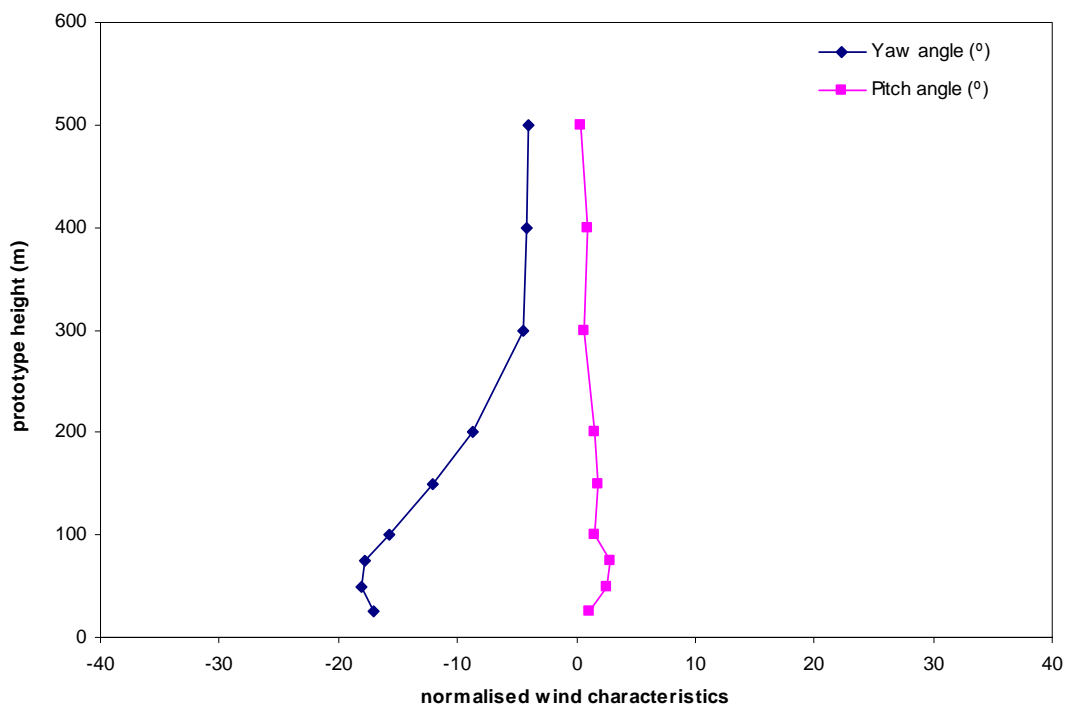
Figure 12b: Mean wind direction, Tsim Sha Tsui, 112.5°
