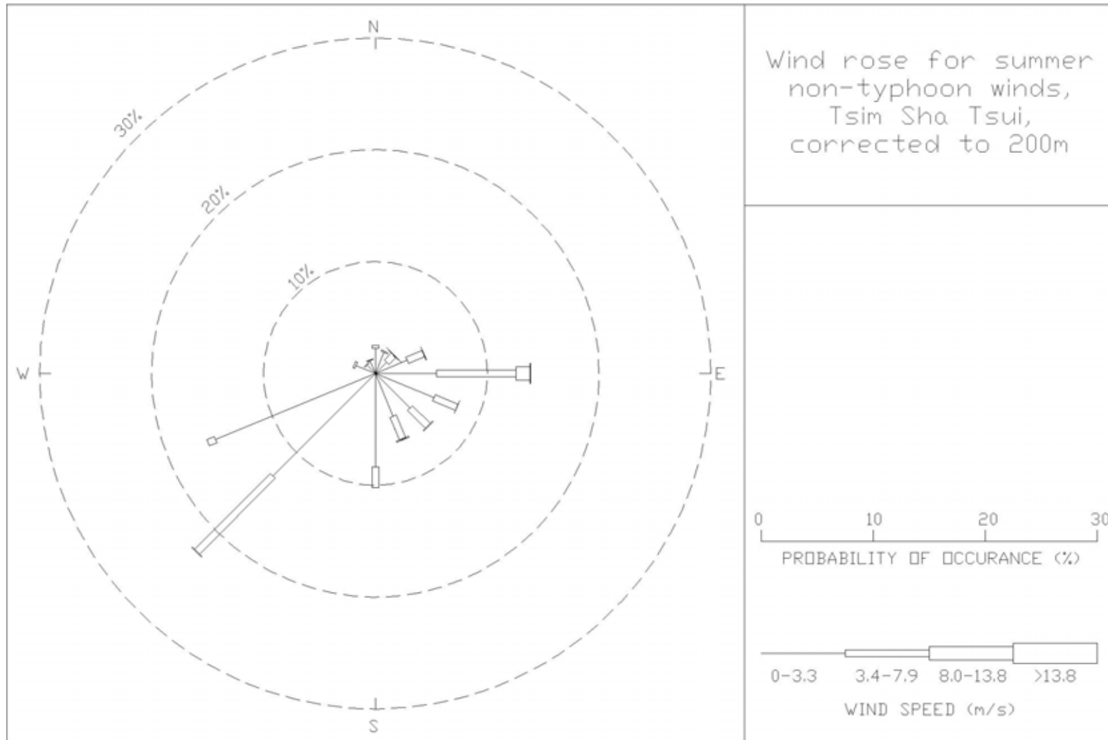
Figure 30: Wind rose for summer, non-typhoon winds for Tsim Sha Tsui, corrected to 200 m
