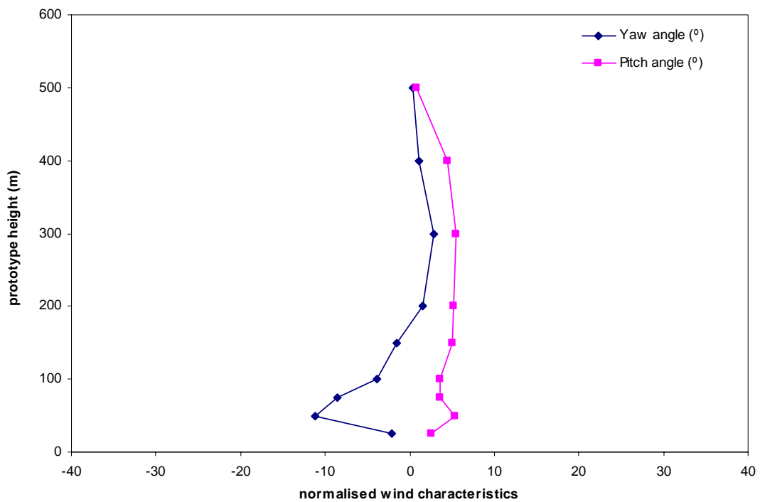
Figure 15b: Mean wind direction, Tsim Sha Tsui, 180°
