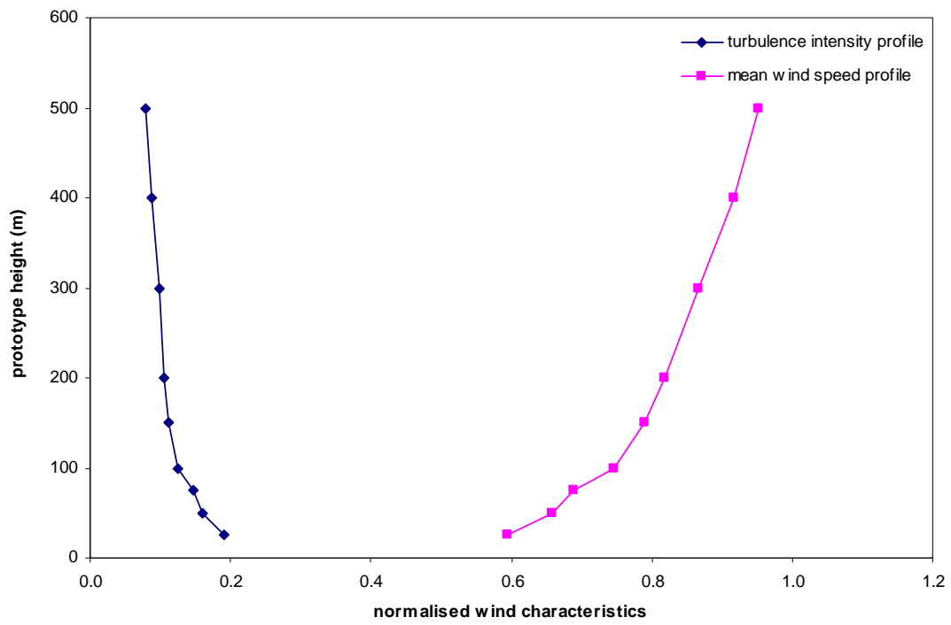
Figure 11a: Wind characteristics, Tsim Sha Tsui, 90°
