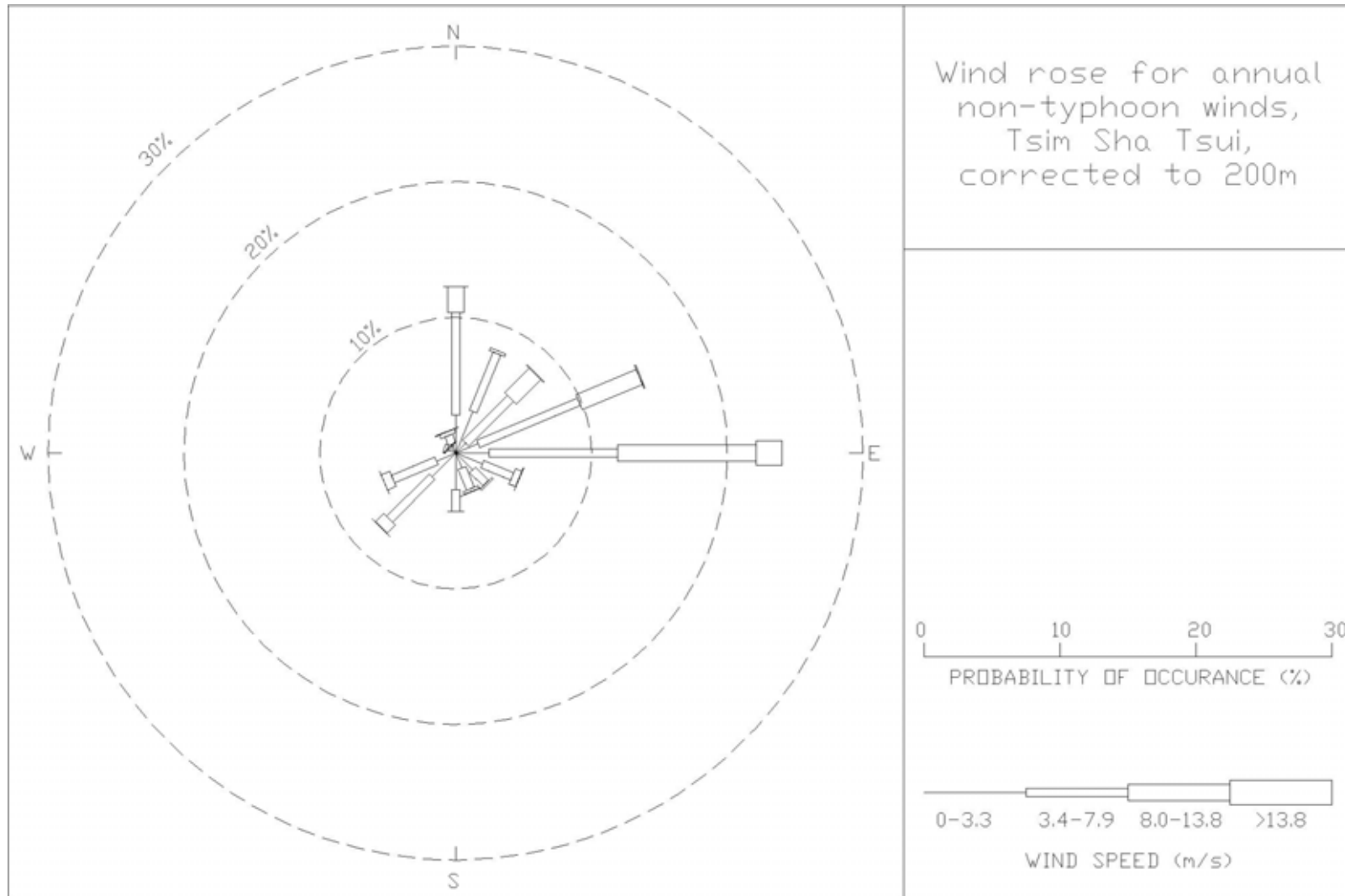
Figure 26: Wind rose for annual, non-typhoon winds for Tsim Sha Tsui, corrected to 200 m
